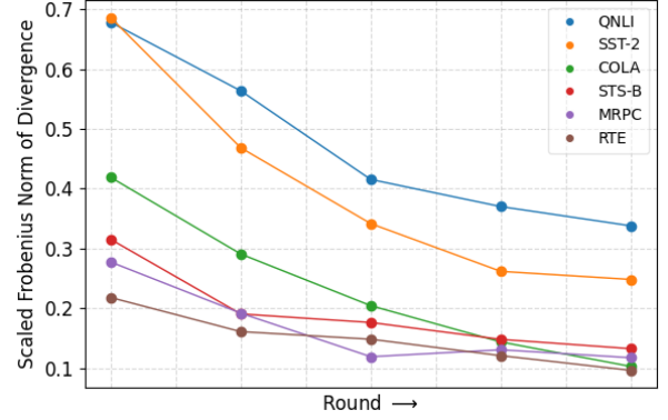
(a) Query matrices of first layer
