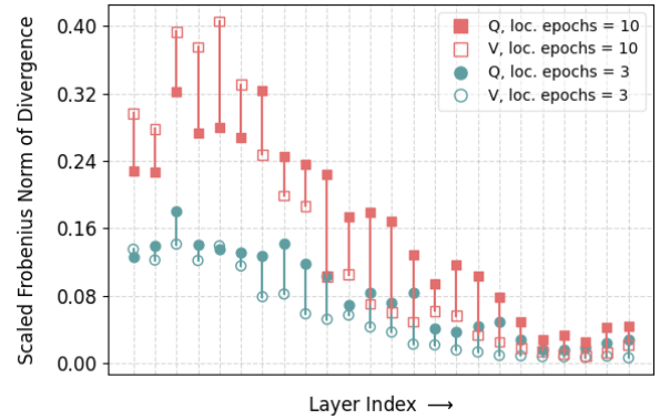
(f) RTE, r = 4
