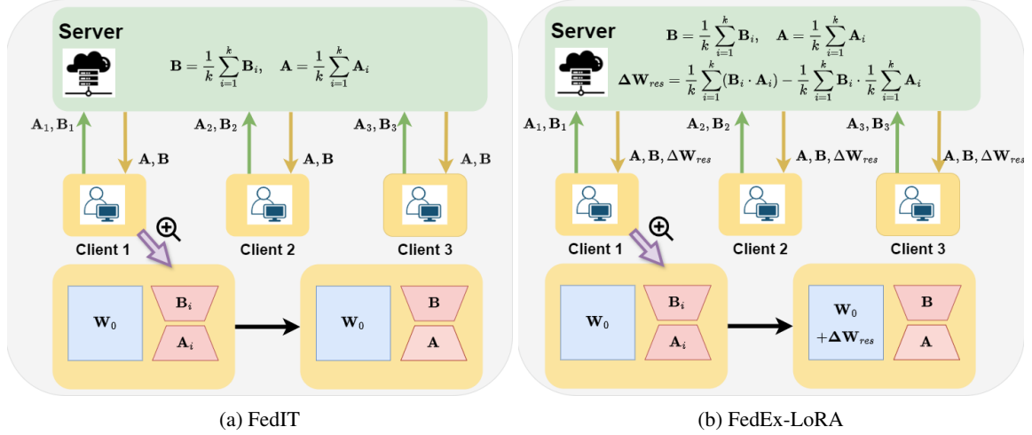
Figure 1: Comparison of federated LoRA methods: (a) FedIT averages the individual client low-rank adapters A_i and B_i , resulting in inexact updates. (b) FedEx-LoRA sends the error residual \Delta W_{res} along with the individual adapters A_i and B_i , which is added to the pretrained weight matrix W_0 , ensuring exact aggregation. Clients transmit low-rank adapters A_i and B_i in both methods.
