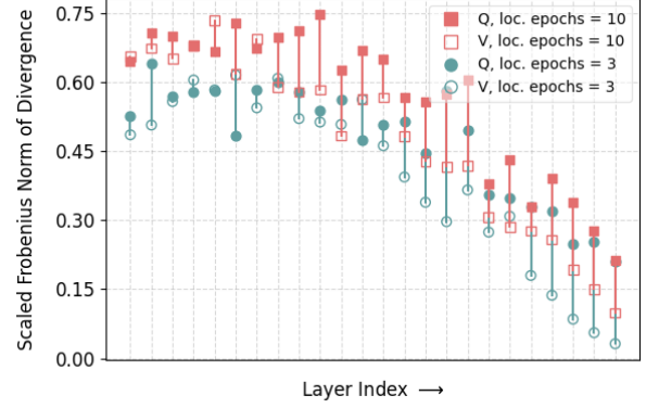
(b) SST-2, r = 4
