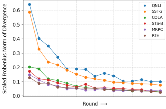
(a) Query matrices of first layer
