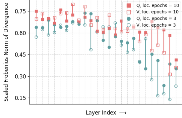
(a) QNLI, r = 4
