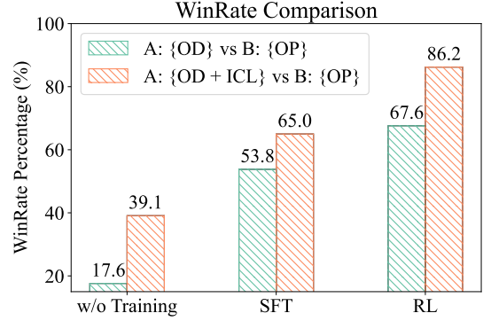
Figure 2: WRs comparison in Vicuna Eval among w/o training, SFT and RL.
