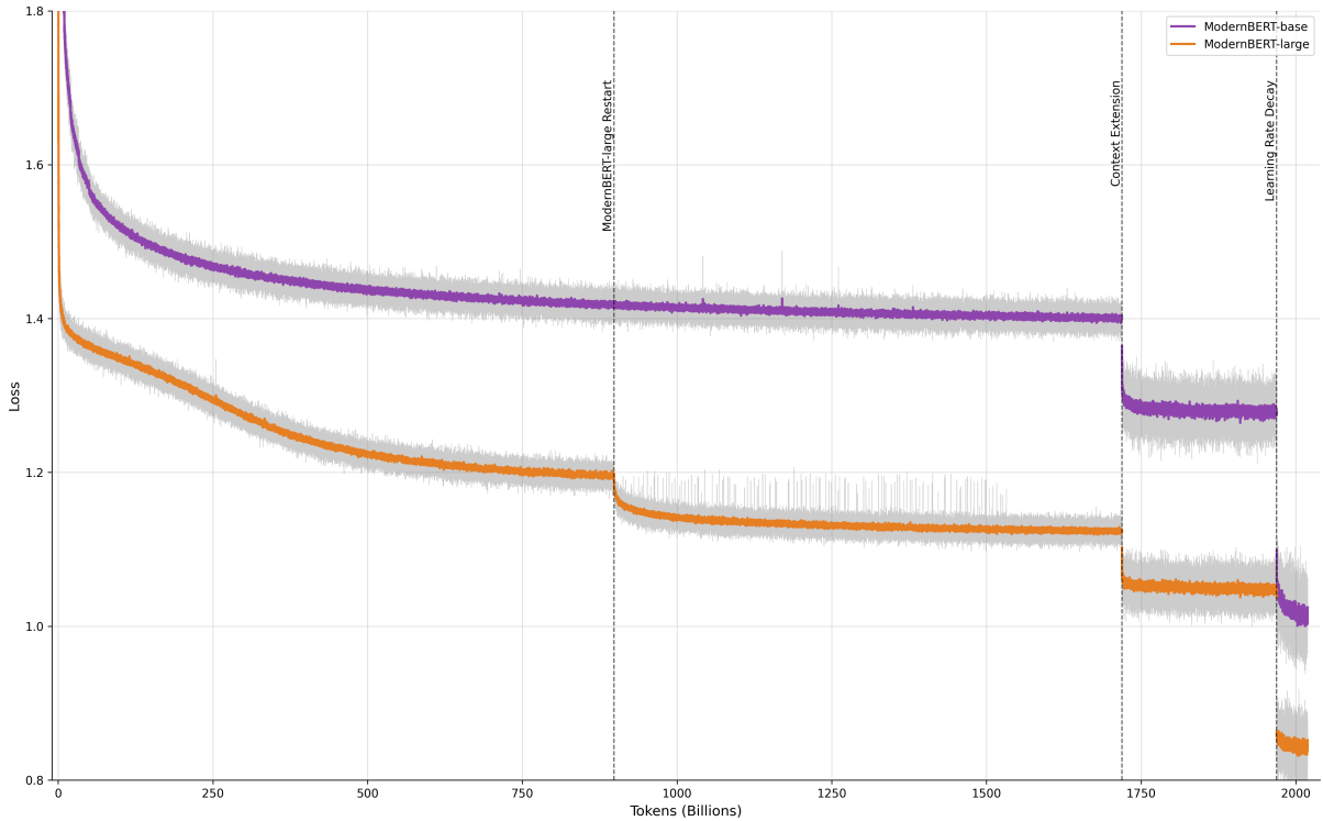
Figure 1: Training loss curves.
