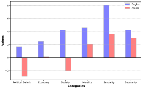
(c) JAIS
