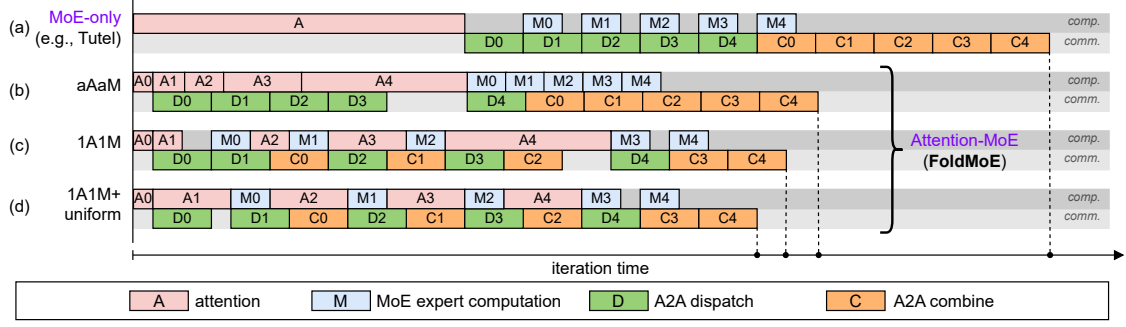
Figure 2: Different token-level overlapping strategies for training a single sequence on one Transformer-MoE block. Computation and communication are on two streams ( comp. and comm. ) to overlap. Existing works (a) pipeline only MoE layer for overlapping. Attention-MoE pipeline in (b) uses an aAaM schedule with large bubbles due to the imbalanced stages (attention and expert computation). FOLDMOE in (c) proposes a 1A1M schedule to reduce these pipeline bubbles by interleaving attention and expert computation. In (d), FOLDMOE additionally uses time-uniform micro-batching to further reduce bubbles caused by imbalanced attention micro-batches, achieving the largest speedup.
