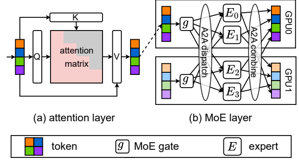
Figure 3: A Transformer-MoE block consists of an attention layer followed by an MoE layer. (b) shows a 4-expert MoE layer with a top-1 gate under 2-way expert parallelism.
