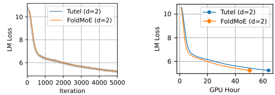
(a) FOLDMOE kept the same logical convergence efficiency as Tutel. The loss curve of both systems
