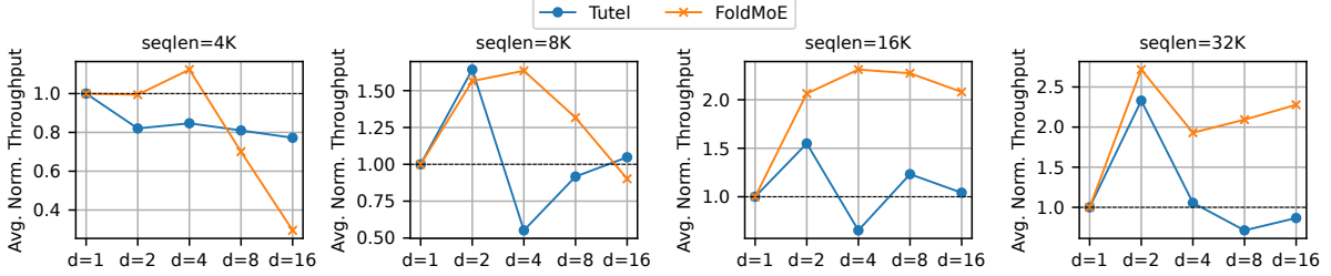
Figure 9: Average normalized throughput of FOLDMOE and Tutel training GPT-MoE-M.
