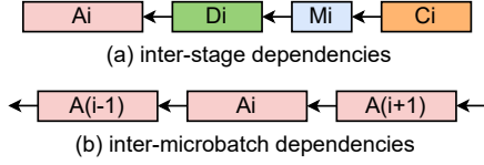
Figure 4: Two categories of data dependencies in the attention-MoE pipeline.
