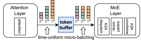
Figure 6: Token buffer between attention and MoE layers to decouple their micro-batching. The sequence can be freely partitioned into micro-batches for time-uniform attention operation, without affecting the MoE layer’s token-uniform micro-batching.
