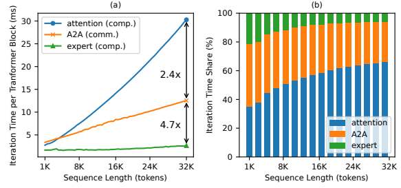
Figure 1: Execution time breakdown of training a GPT-MoE model on 2 AWS g5.24xlarge instances (each with 4 NVIDIA A10G GPUs)
