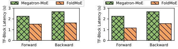
Figure 10: Latency of forward and backward pass of Transformer-block in GPT-MoE-M with 32K seqen. Left: d=2 . Right: d=8 .
