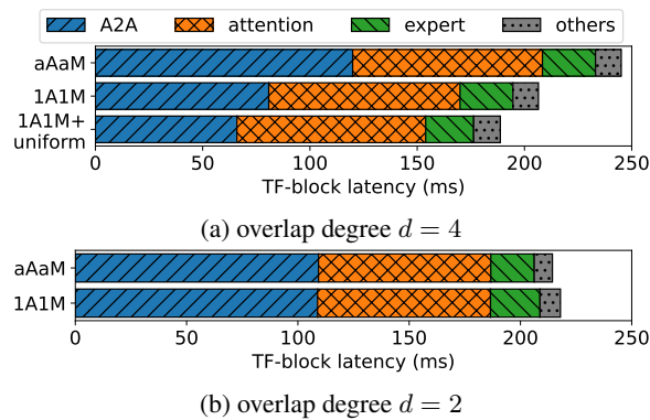
Figure 11: Breakdown of average Transformer block latency on critical path of training GPT-MoE-L on 32K seqen with different FOLDMOE scheduling.
