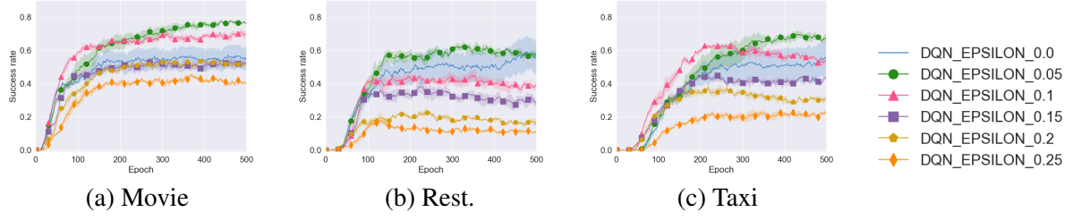
Figure 7: Effect of epsilon parameters on DQN performance
