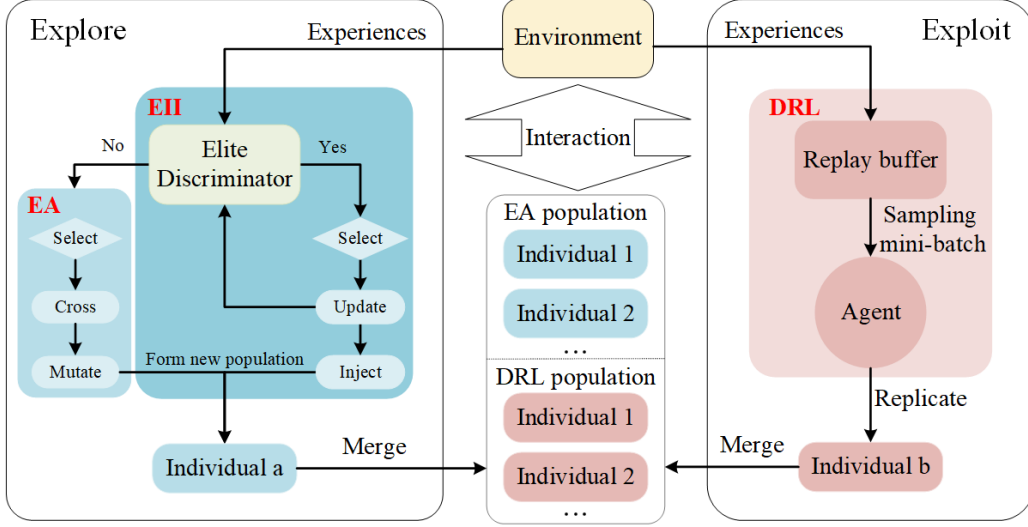
Figure 1: Framework of the EIERL method, comprising two modules: exploration and exploitation. The exploration module aims to form an EA population (multiple individuals a) to explore diverse experiences, while the exploitation module aims to form a DRL population (multiple individuals b) to use existing experiences for training.
