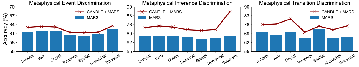
Figure 4: Performances by component types of fine-tuned LLaMa3-8B on three tasks of MARS.
