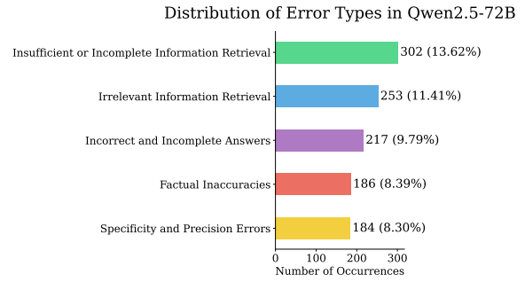
Figure 11: The statistics of fine-grained RAG error types in Qwen2.5-72B.
