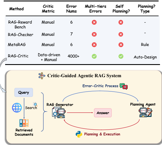
Figure 1: The comparison between RAG-Critic and other methods (Upper part). The overview of our Critic-Guided Agentic RAG framework (bottom part).
