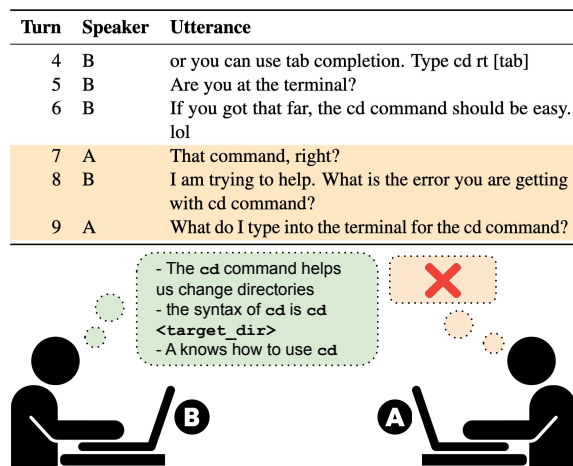
Figure 1: An annotated instance of conversational friction. Though it is challenging to access propositions in a speakers’ perception of common ground, certain propositions in B’s version of common ground are revealed (green thought bubble) when there is a misalignment between the two participants. B assumes A knows about the cd command, which is proven false by A in Turn 9.
