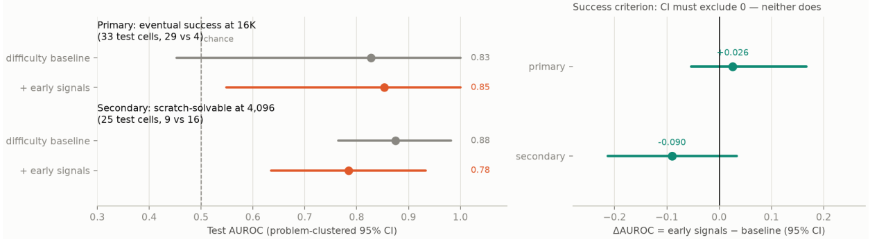
Figure 5: The confirmatory test: single evaluation on the held-out split. Neither endpoint’s \Delta AUROC CI excludes zero.
