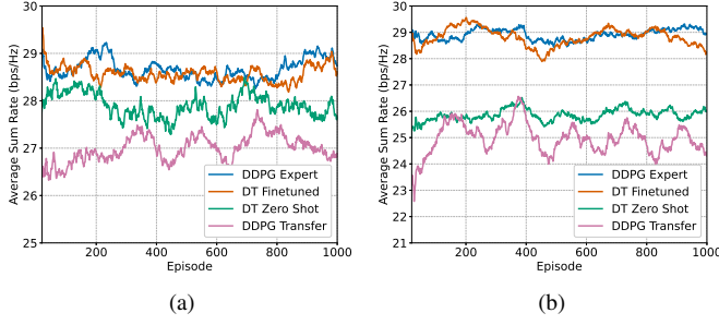
Fig. 4: Evaluation results of the DDPG expert, fine-tuned DT, zero-shot DT, and transferred DDPG policies in the unseen scenario. (a) Initial UAV-mounted RIS position at [15,15,4.5]. (b) Initial UAV-mounted RIS position at [25,25,4.5].
