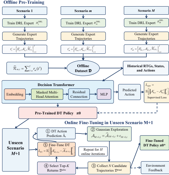
Fig. 2: Decision Transformer Framework with Offline Pre-Training and Online Fine-Tuning
