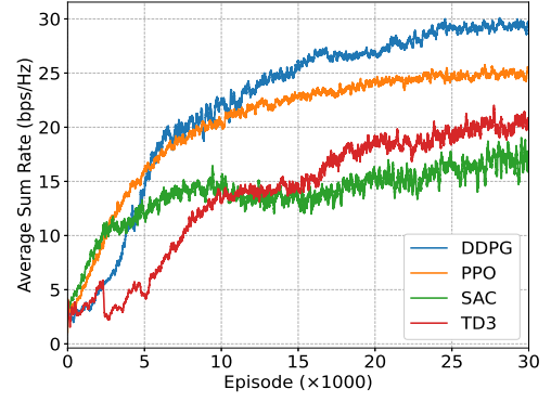
Fig. 3: Convergence performance comparison of different DRL algorithms in the UAV mounted RIS-assisted communication environment.
