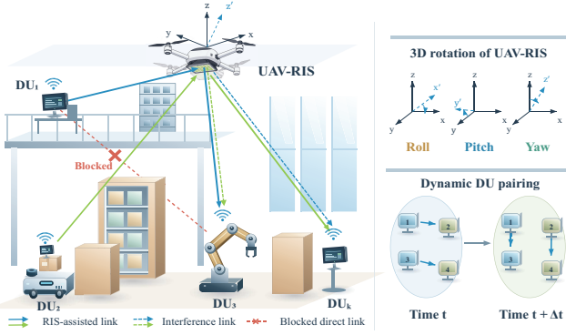
Fig. 1: UAV-Mounted RIS-Assisted Dynamic D2D Communication System.
