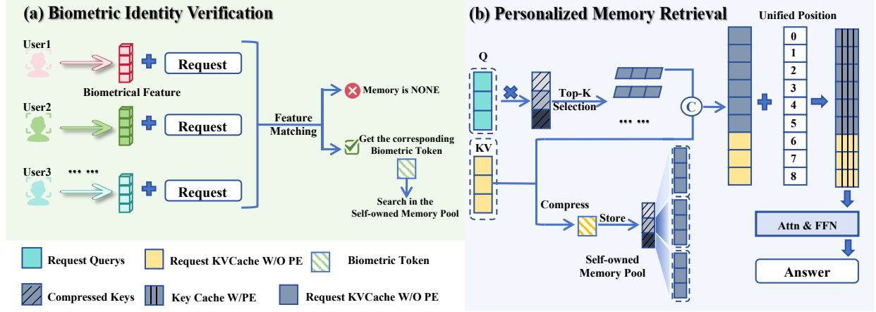
Figure 1: Overall pipeline of Bio-MemArt. (a) Biometric identity verification matches the current user’s biometric feature against enrolled identities and activates only the corresponding owner memory pool; unmatched requests receive no authorized memory. (b) Personalized KV-memory retrieval is then performed inside the authorized candidate pool: the request is encoded into query KV states, compressed keys are used for top- K block selection, selected memories are merged under a unified position layout, and the decoder reuses the retrieved KV cache to generate the final answer.
