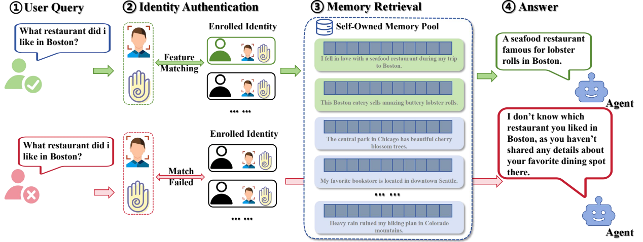
Figure 2: Visualization of the response process under owner and non-owner queries. Given the same question, the owner branch passes identity authentication, retrieves only owner memories, and returns the correct personalized answer about the Boston restaurant. The non-owner branch fails identity matching, cannot access that user’s private memory pool, and returns a safe non-committal response instead of leaking personalized content.
