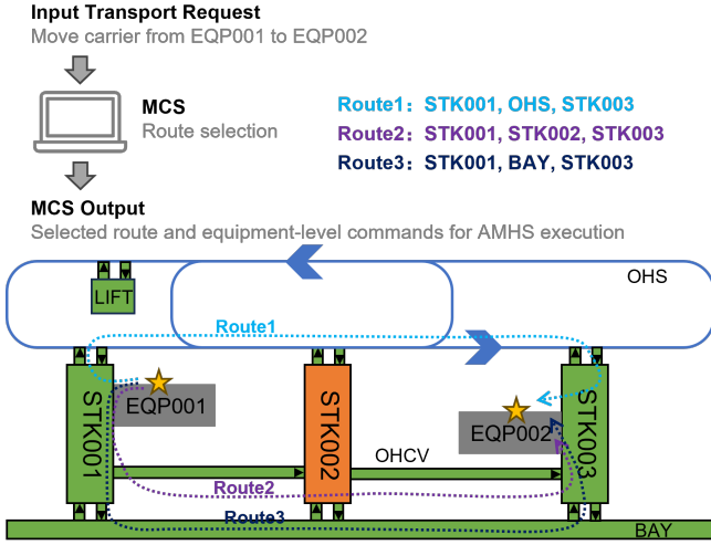
Fig. 1. Illustration of congestion-aware route selection in the MCS. The MCS compares multiple feasible routes for transferring a carrier from EQP001 to EQP002. The orange STK002 denotes a congested stocker with many queued commands, which may increase the delivery delay of Route 2. The example shows why route evaluation should consider current congestion exposure at relay resources as well as static route length.
