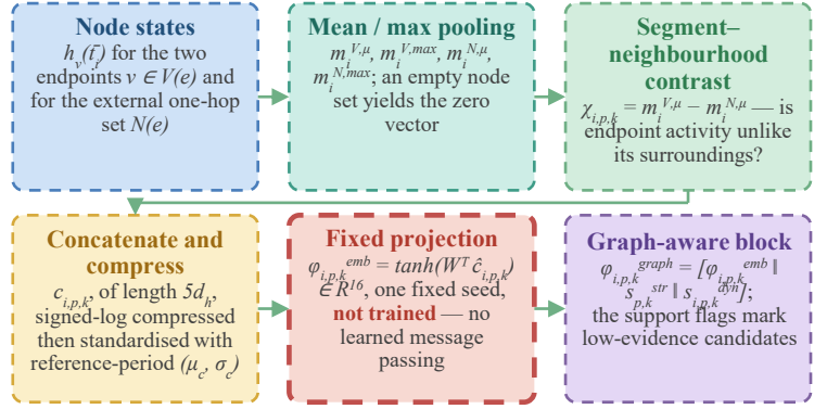
(b) From node states to the graph-aware block \phi^{graph}
