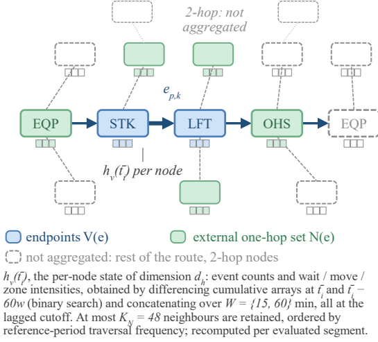
Fig. 4. Graph-aware edge representation. Endpoint and neighboring-node states are mean/max pooled and contrasted, transformed by a fixed untrained projection, and concatenated with structural and dynamic support diagnostics.
