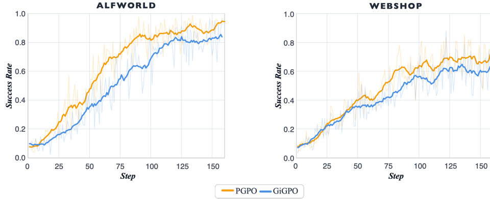
Figure 7: Training curves of PGPO and GiGPO on ALFWorld (left) and WebShop (right).
