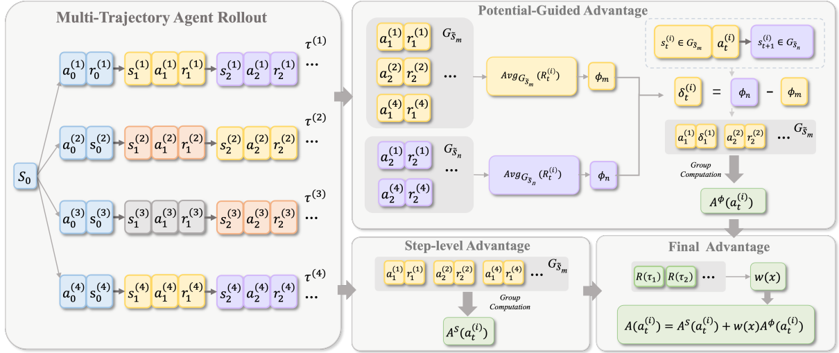
Figure 2: Overall pipeline of PGPO. Given a rollout group, PGPO constructs anchor-state groups across trajectories, estimates empirical state potentials from outcome-derived step returns, computes a potential-guided advantage from one-step potential differences, and combines it with the step-level advantage through task-level success-adaptive weighting. The displayed potential difference uses the default setting \gamma = 1 .
