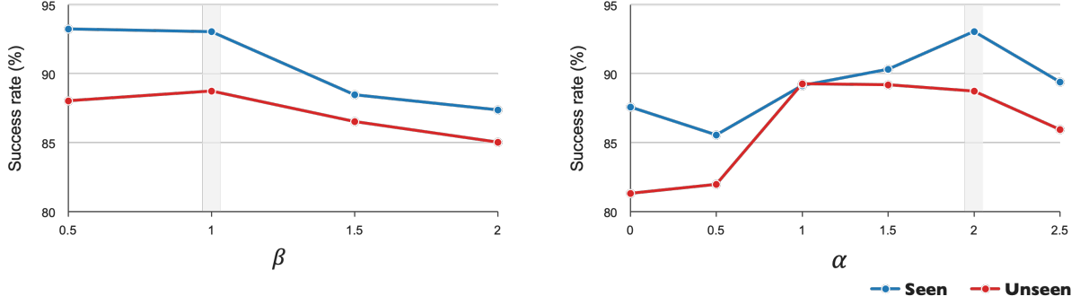
Figure 6: Sensitivity of PGPO to \beta and \alpha on ALFWorld. The shaded regions mark the default settings used in the main experiments.
