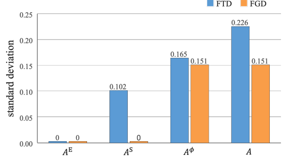
Figure 3: Failure-side discrimination on ALFWorld training rollouts. A is the final PGPO advantage; higher FTD and FGD indicate stronger local differentiation among failed steps.
