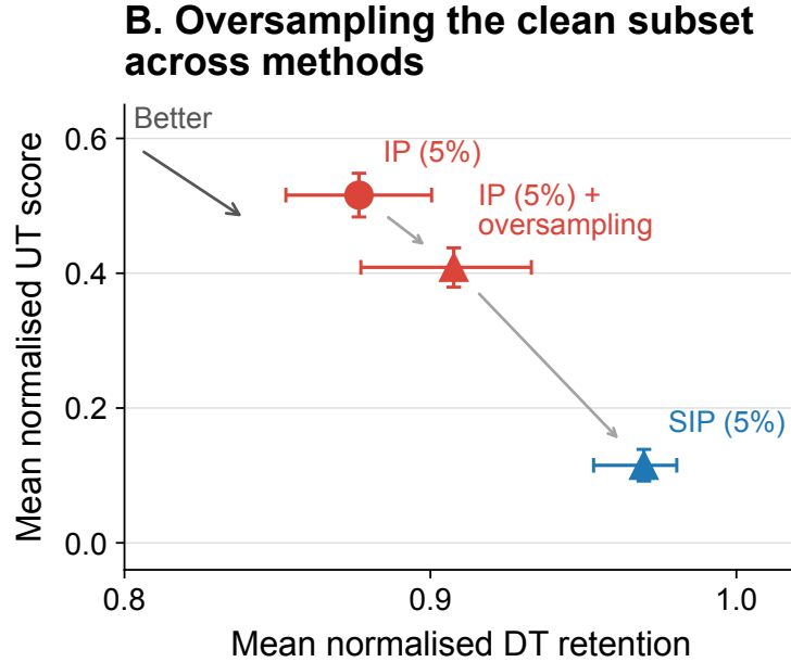
Figure 7: Oversampling across methods with confidence intervals. Expanded view of Figure 3B. All three conditions use the same distinct 5% clean subset. Standard IP assigns 5% of training positions to clean examples; oversampled IP and SIP assign 25%. The total number of training positions is fixed. Oversampled IP and SIP match training examples, sampling frequencies, and optimisation settings, differing only in the prompts assigned to clean examples. Scores are normalised within each setup and averaged equally across six setups, with three training seeds per condition. Horizontal and vertical error bars show 95% confidence intervals from 5,000 bootstrap draws over training seeds and question clusters, including uncertainty in the normalisation anchors. See Appendix B for statistical details.
