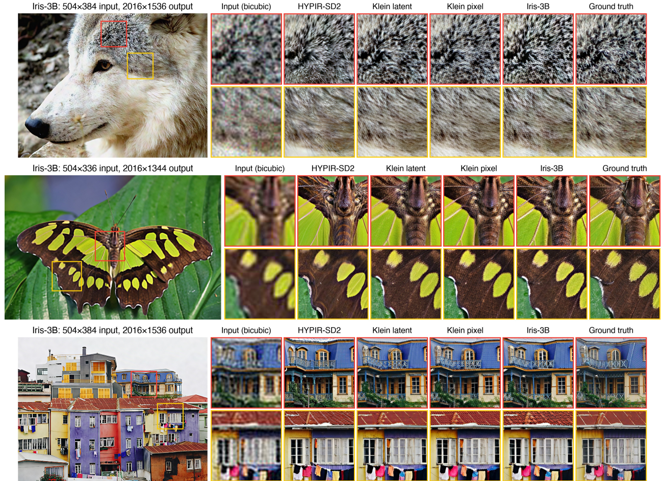
FIG. 10 4x restoration of further DIV2K validation images with native Real-ESRGAN degradations (the Tab. 6 pairs).
