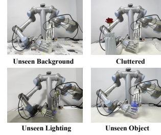
Figure 8: OOD scenarios.
