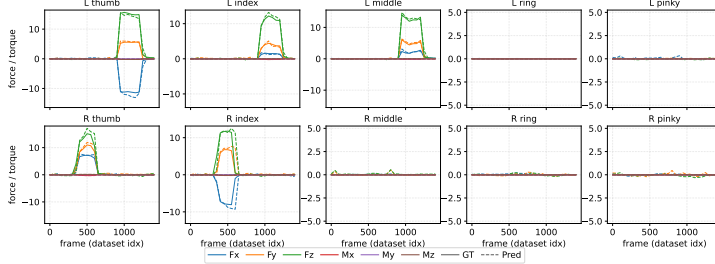
Figure 7: Force prediction.
