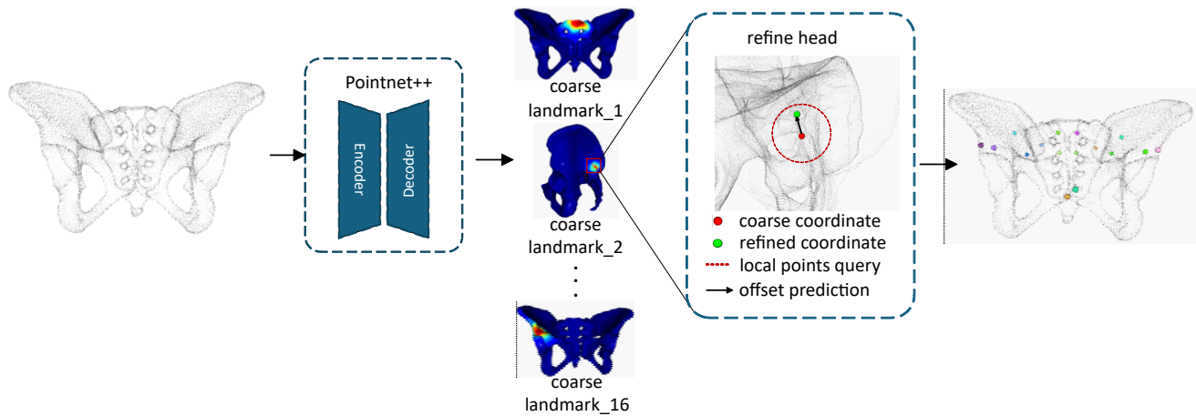
Figure 3.4. Architecture of the landmark detection network.
