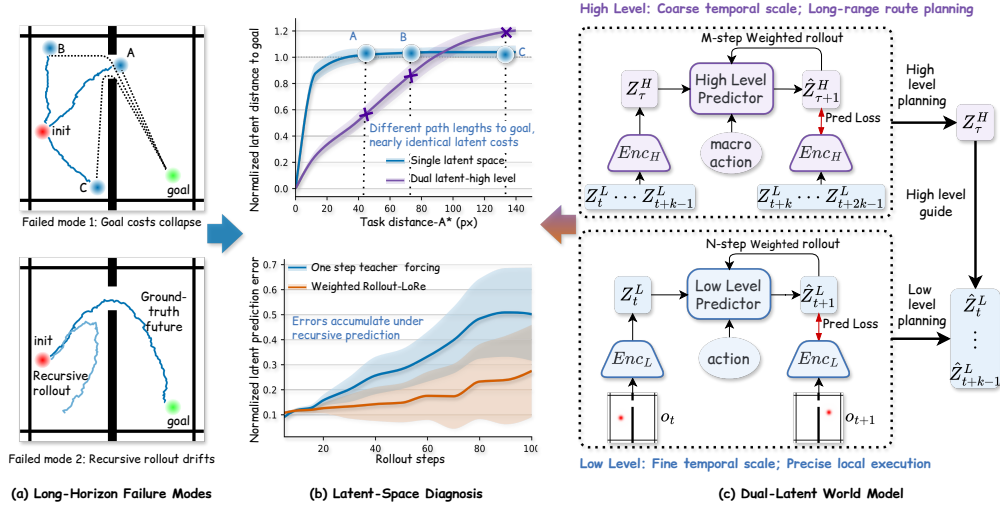
Figure 1: Overview of the long-horizon planning problem and our dual-latent solution. (a) Two failure modes in a single latent space: goal costs collapse for distant states, and recursive rollouts drift from the ground-truth future. (b) Latent-space diagnostics: the high-level space preserves task-distance contrast, while weighted rollout training reduces multi-step prediction error relative to one-step teacher forcing. (c) Dual-WM assigns coarse route planning to a high-level latent and precise local execution to a low-level latent.
