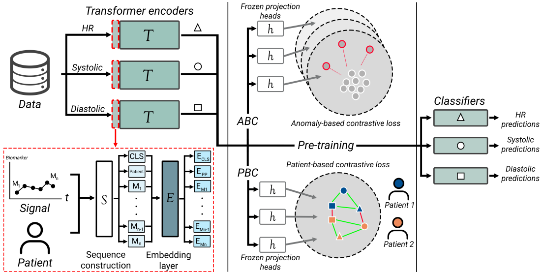
Fig. 4: Illustration of the model architecture. The model is divided into three parts: transformer encoders (left), pre-training (middle) and classification networks (right). The embedding process is shown in the red-striped box. The tokenized measurement sequence is shown as boxes labeled M_i and embeddings are shown as boxes labeled E_i . Each biomarker is illustrated as a different geometrical shape as the output from the encoders. For ABC pre-training (top), each representation is projected into a specific feature domain where the hospitalized windows (red) are separated from the non-hospitalized windows (white). For PBC pre-training (bottom), all representations are projected into the same domain where each window from the same patient is regarded as a positive pair (green link) and each window from different patients is seen as a negative pair (red link). Abbreviations: t = Time, HR = Heart Rate, SYS = Systolic Blood Pressure, DIA = Diastolic Blood Pressure, M = Measurement
