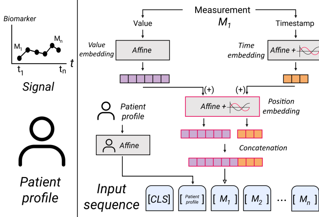
Fig. 5: Illustration of the embedding process. The sources of information are shown to the left. Measurement M_1 in the figure is decomposed into a value and a timestamp. The value undergoes affine transformation to produce a value embedding, whereas the timestamp is converted into a time embedding with sinusoidal encoding. These are then further transformed to form position-aware embeddings followed by concatenation. The patient profile is independently embedded through an affine layer. All components: a CLS -token, the patient profile, and the measurement embeddings are concatenated to form the input sequence.
