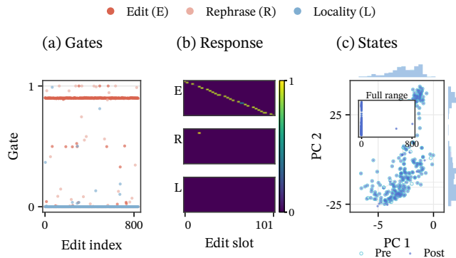
Fig. 3. Runtime behavior after 839 CounterFact edits on Llama-3.1-8B-Instruct. (a) Matched-slot gates for edits and rephrases, and the maximum gate for locality queries. (b) Responses of the first 32 sampled queries to their associated slots. (c) Paired final-block locality states under shared PCA, with empirical marginals and a full-range inset. PC1/PC2 explain 45.1%/10.7%; mean relative state drift is 11.54% and next-token agreement is 96.5%.
