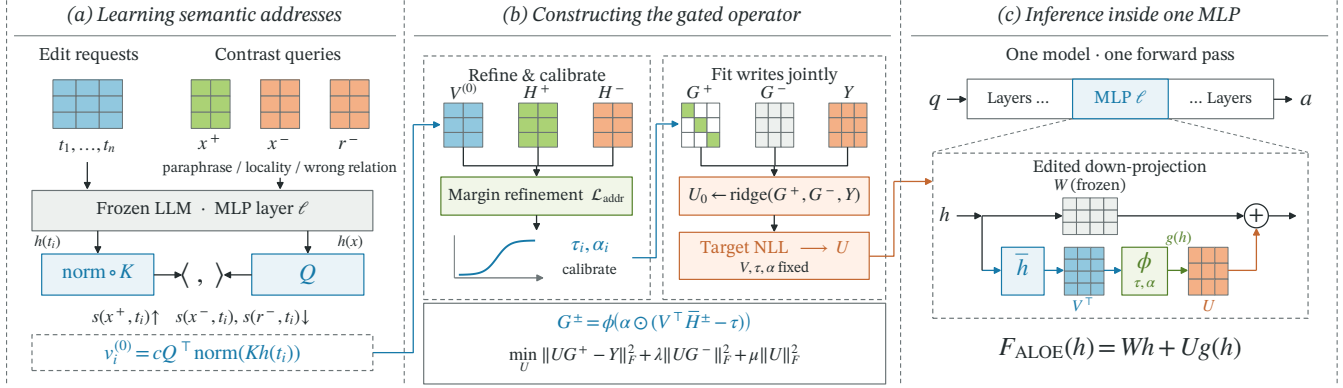
Fig. 2. ALOE learns semantic addresses, refines and calibrates continuous edit gates, and inserts the resulting low-dimensional residual into one MLP projection. The edited LLM executes the operator in a standard forward pass.
