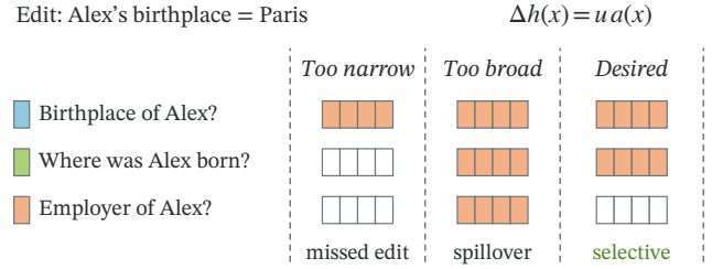
Fig. 1. The address problem. The same write can miss paraphrases or affect neighboring facts. Filled cells denote an active write; empty cells denote no update (schematic).
