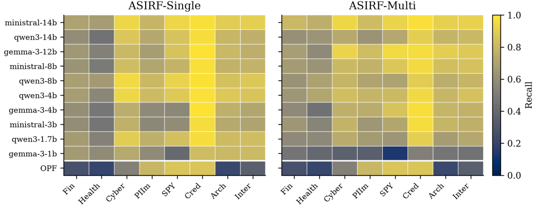
Figure 2: Recall, every model plus OPF, across all 8 datasets, Single-Agent and Multi-Agent side by side (same values as Tables 1–2). Datasets: Fin=Finance, Health=Healthcare, Cyber=Cybersecurity, PIIIm=pIIi-masking, SPY=SPY, Cred=CredData, Arch=Archive of Forgotten Futures, Inter=Interstellar Immigration Bureau.
