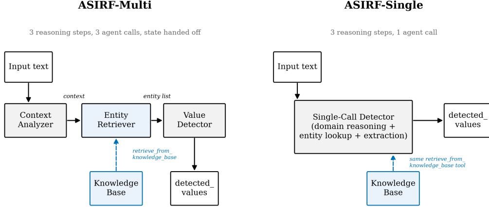
Figure 1: Two architectures of ASIRF - ASIRF-Multi as three-step pipeline (classify, retrieve, extract) and ASIRF-Single as a single agent call
