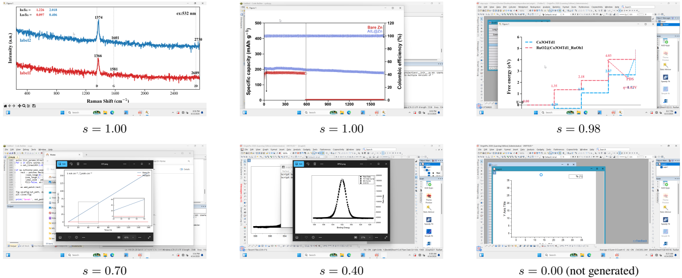
Figure 9: Representative Origin figures generated by Claude Sonnet 4.6 with script+hint (top) and no_script+no_hint (bottom). Scores are computed as s = (C + A + T)/(3 \times 5) . Template scripts produce high-quality outputs ( s \geq 0.98 ), whereas GUI-only execution reduces quality ( s \leq 0.70 ) or fails ( s = 0 ).
