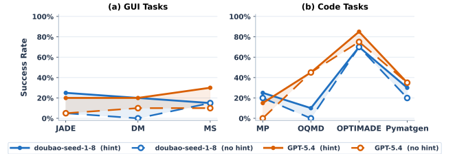
Figure 4: Ablation study: SR comparison between hint (solid) and no_hint (dashed) prompt modes for Doubao-seed-1-8 (blue) and GPT-5.4 (orange). Left: GUI tasks. Right: Code tasks. Shaded bands indicate the gap between hint and no_hint conditions.
