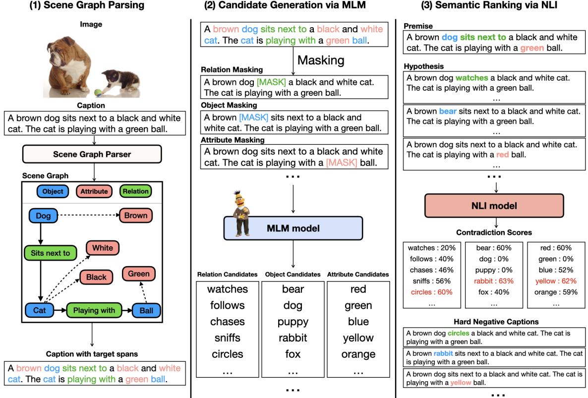
Figure 3: Overview of CS-CLIP. Our framework generates hard negatives in three steps: (1) identifying compositional elements via scene graph parsing, (2) generating candidates with an MLM, and (3) selecting contradictory captions using an NLI model.
