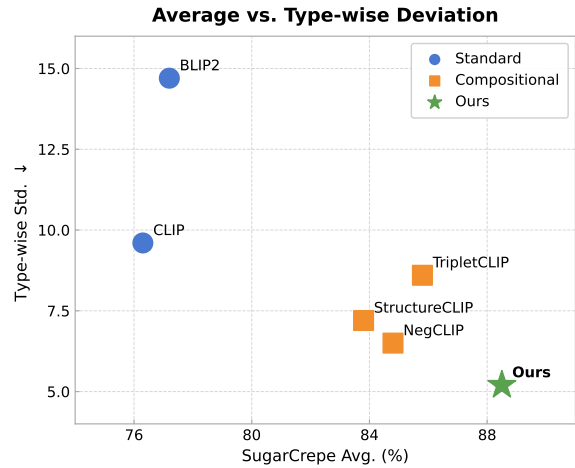
Figure 1: Average performance versus type-wise deviation on SugarCrepe. CS-CLIP (Ours) achieves the highest SugarCrepe average with the lowest standard deviation across reasoning types, indicating more robust compositional reasoning.
