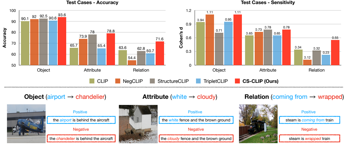
Figure 2: Results of our controlled evaluation. We illustrate the accuracy and sensitivity metrics for each element (top) and present representative cases of positive and hard negative captions (bottom).
