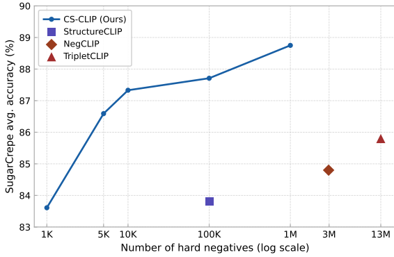
Figure 5: Sample efficiency of CS-CLIP on SugarCrepe. CS-CLIP is trained across data scales from 1K to 1M hard negatives. Baseline checkpoints are placed at their reported training scales.
