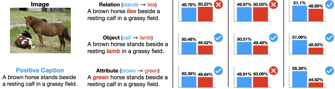
Figure 4: Qualitative analysis. We present an image with its corresponding positive and negative captions, along with prediction probabilities across models. ✓ (blue) and ✗ (red) denote correct and incorrect answers, respectively. Compared to CLIP and TripletCLIP, CS-CLIP demonstrates a clearer margin in distinguishing compositional element changes and selects the correct answers.
