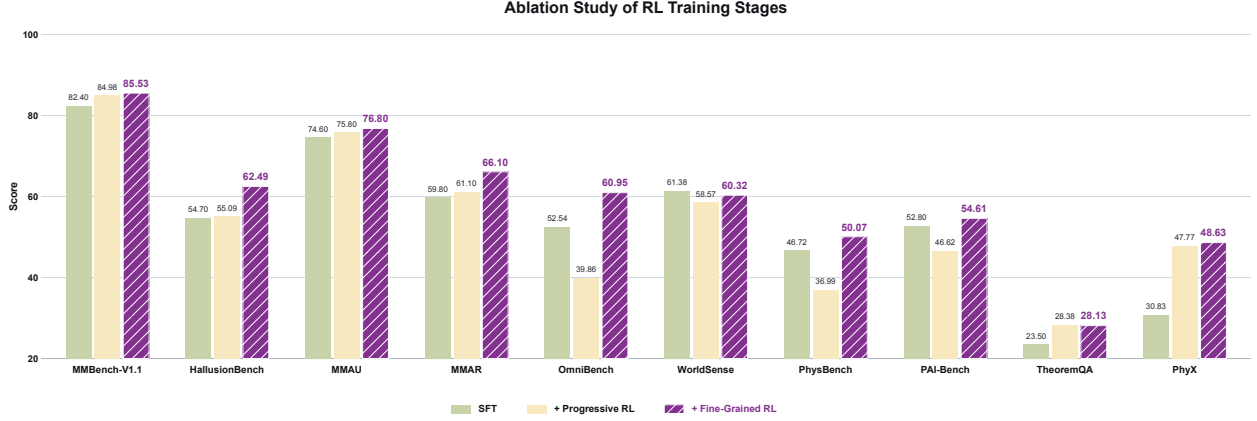
Figure 10 Successive checkpoints across ten understanding and reasoning benchmarks. SFT denotes the Stage 1-3 checkpoint; Progressive RL adds Stage 2-1 answer-correctness optimization; Fine-Grained RL further adds Stage 2-2 physical-perception and format rewards. Each row continues training from the preceding row. Higher scores are better.
