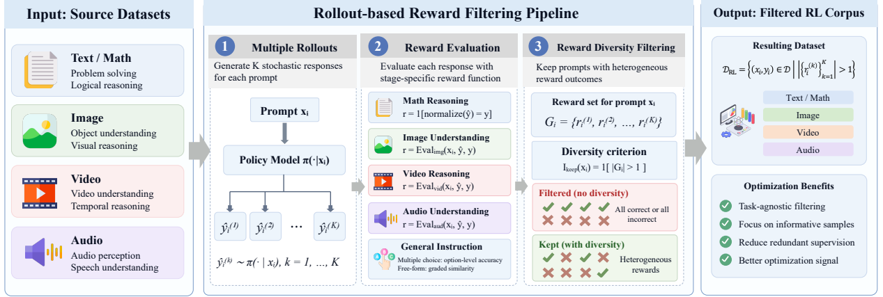
Figure 5 Rollout-based reward-diversity filtering for RL data curation. For each prompt, a fixed policy generates K stochastic responses ( K = 4 by default), which are scored by task-specific reward evaluators. A prompt is retained only if its rollout group contains more than one distinct reward value. Uniform-reward groups are discarded; for binary rewards, these correspond to all-correct or all-incorrect responses. The retained corpus provides within-group reward variation for subsequent GRPO training.
