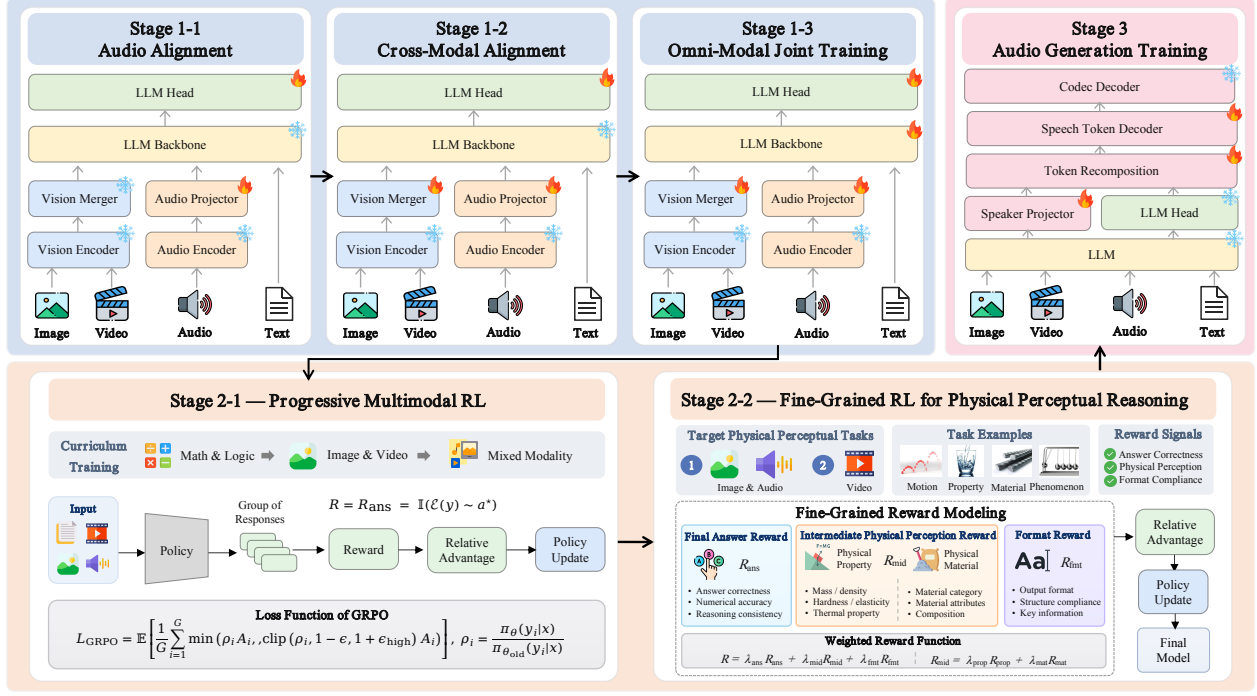
Figure 7 Training curriculum of OmniPhysics-Nano-V2. Stage 1 comprises Audio Alignment (Stage 1-1), Cross-Modal Alignment (Stage 1-2), and Omni-Modal Joint Training (Stage 1-3). Stage 2 first performs Progressive Multimodal RL with answer-level rewards (Stage 2-1), then applies Fine-Grained RL for Physical Perceptual Reasoning with final-answer, intermediate-perception, and format rewards (Stage 2-2). Stage 3 performs Audio Generation Training while keeping the multimodal reasoner and codec decoder frozen. Flame and snowflake symbols denote trainable and frozen components, respectively.
