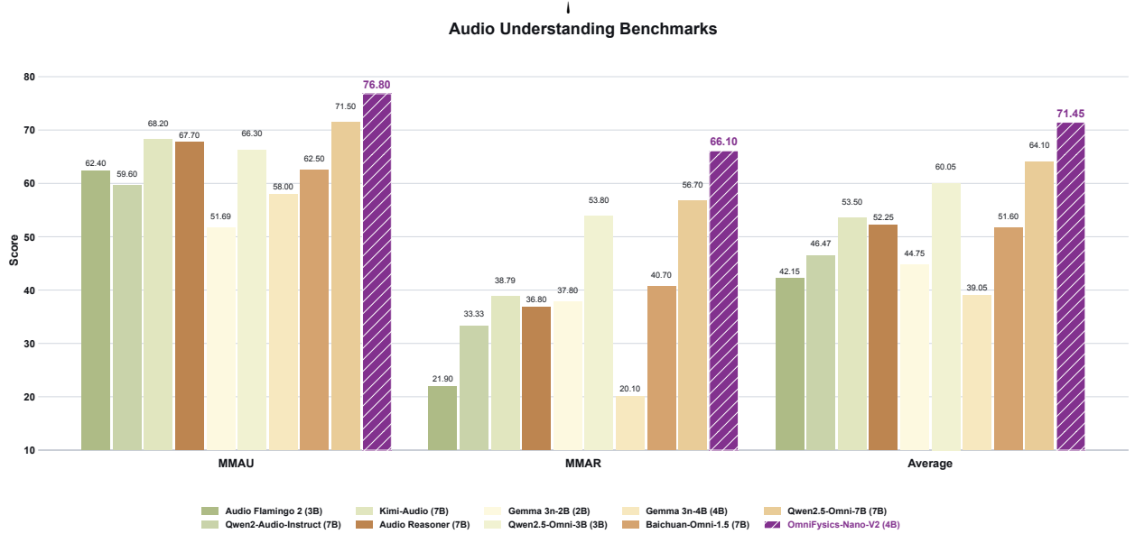
Figure 8 Comparison of Audio Understanding Performance on MMAU and MMAR. Purple hatched bars denote our model.
