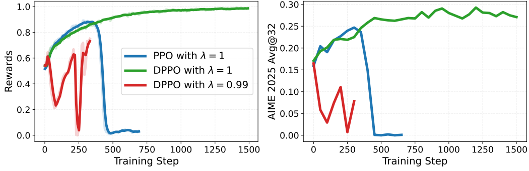
Figure 1: PPO and DPPO in the sanity test. With \lambda = 1 , PPO’s training reward collapses after an initial increase, whereas DPPO remains stable. Reducing the GAE parameter to \lambda = 0.99 makes DPPO unstable and exposes sensitivity to critic error.
