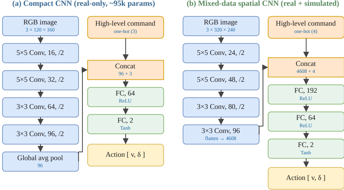
Figure 1. Policy architectures. (a) The compact command-conditioned CNN baseline (94,882 parameters): a convolutional encoder with global average pooling whose embedding is concatenated with the one-hot command and decoded by a two-layer MLP. (b) The larger command-conditioned variant: a spatial encoder whose flattened features are concatenated with the command and decoded by a three-layer MLP.
