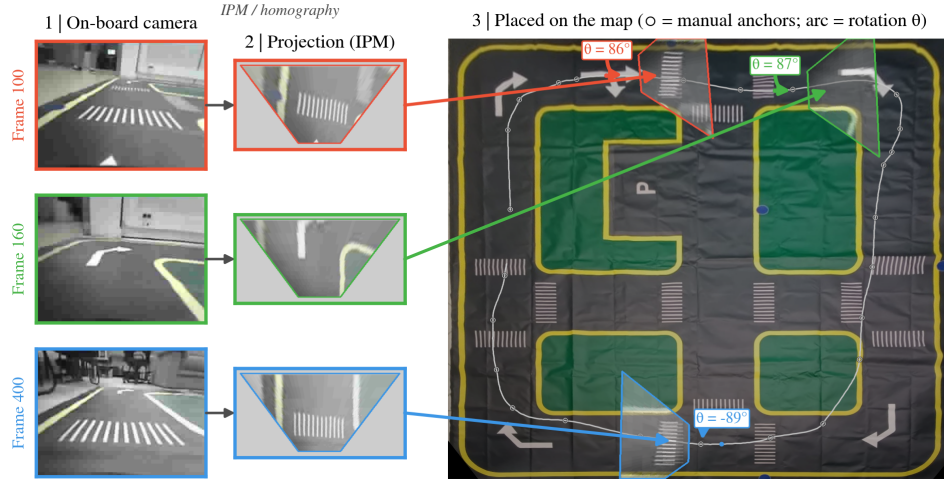
Figure 6. Map-registered localization of an outer-loop run: per-frame camera images are projected to the ground plane and the reconstructed trajectory is overlaid on the rectified map, illustrating the registration behind the cross-track-error metric.
