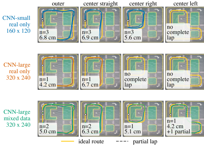
Figure 7. Comparison of map-registered neural-control laps by policy variant. Each row groups the autonomous runs from one policy; columns show the four route loops. Colored lines are registered real-robot laps, dashed lines are partial laps, yellow lines are ideal routes, and each panel reports the mean cross-track error over complete laps.
