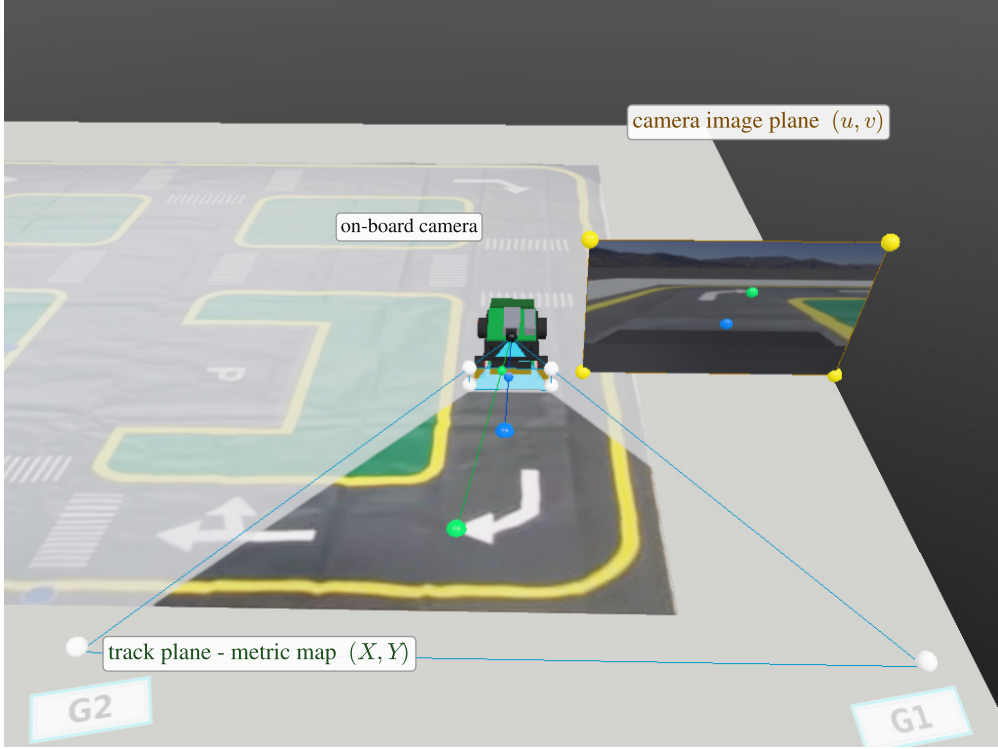
Figure 5. Ground-plane homography. Because the track is planar, camera intrinsics and pose define a single 3 \times 3 homography between metric map coordinates (X, Y) and image pixels (u, v) . The projection tool uses this mapping, or its inverse, to relate on-board camera observations to the rectified map; the figure illustrates the geometry in the Webots digital twin. The blue and green markers are the same physical points on the track and in the camera image.
