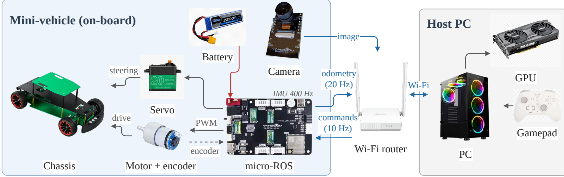
Figure 2. Experimental setup, split into the on-board mini-vehicle and the host PC: the ESP32-S3 micro-ROS board closes the 100 Hz speed PID loop and drives the servo, while a separate ESP32 camera streams images to the host PC, which runs the policy and the extended Kalman filter and returns steering and speed commands.
