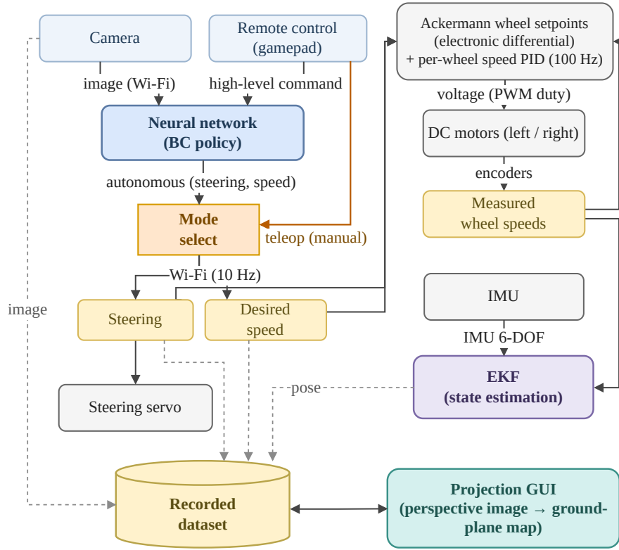
Figure 4. End-to-end signal flow. During data collection a human teleoperates the vehicle and the mode-select logs the commanded steering/speed—with the camera image and the EKF pose—into the recorded dataset; at deployment the behavior-cloning policy replaces the teleoperator, producing steering and a speed setpoint; on board, steering drives the servo and, with the speed setpoint, defines per-wheel setpoints (Ackermann electronic differential) for the 100 Hz PID loops, while the projection GUI maps recorded images to the ground plane.
