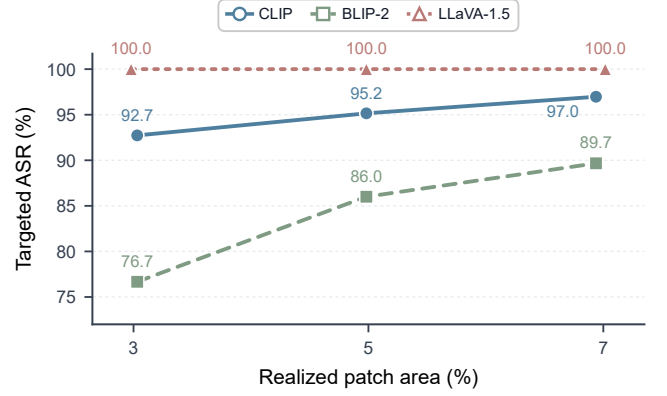
Figure 4: Targeted ASR as a function of realized patch area for the representative classification, conditional-generation, and binary-VQA variants.
