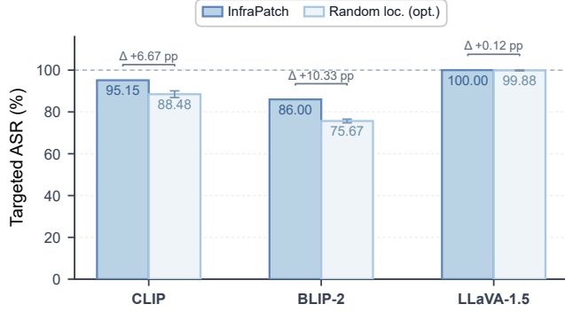
Figure 3: Targeted ASR under full InfraPatch and optimized random placement. Error bars denote sample standard deviation across three seeds.
