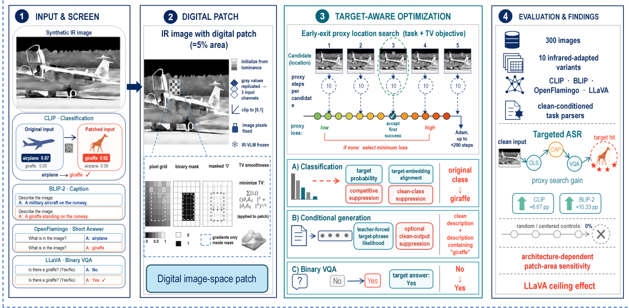
Figure 1: InfraPatch pipeline. Given a clean DiffV2IR-translated image and a fixed target semantic, the method first evaluates candidate patch locations through early-exit proxy search. It then refines the selected grayscale patch with a task-specific objective for classification, conditional generation, or binary VQA, and returns the adversarial output under the corresponding success rule.
