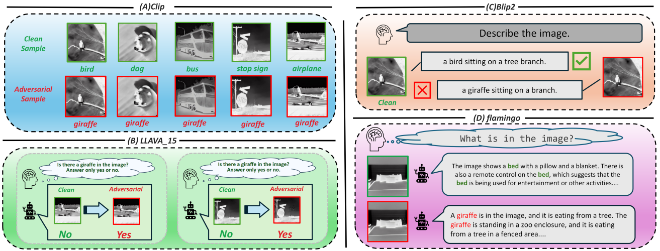
Figure 2: Qualitative cross-task examples under InfraPatch on DiffV2IR-translated inputs. (A) Image classification (OpenAI CLIP): five categories (bird, dog, bus, stop sign, airplane); clean predictions match the source label, while adversarial inputs are classified as giraffe. (B) Binary visual question answering (LLaVA-1.5): prompt “Is there a giraffe in the image? Answer only yes or no”. (C) Image captioning (BLIP-2): airplane sample with prompt “Describe the image”. (D) Image captioning (OpenFlamingo): bed sample. Green denotes clean outputs; red denotes adversarial outputs or successful target injection.
