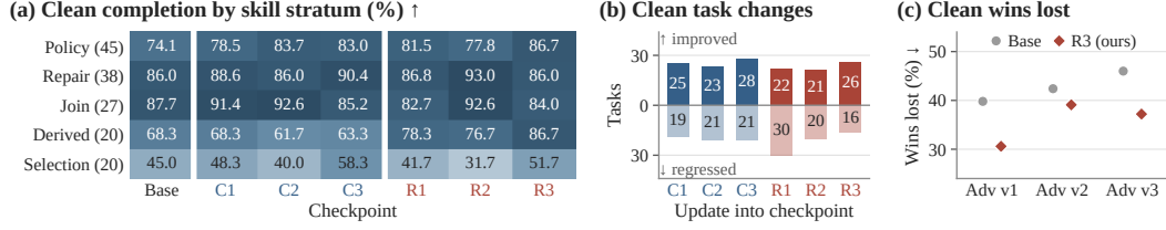
Figure 5: Clean completion by stratum, task changes per update, and clean wins lost under attack. (a) Clean judged completion (%) by skill stratum and checkpoint, mean over three seeds; task counts in parentheses. (b) Tasks whose number of good judgments over the three seeds increases or decreases after each update (ties omitted). (c) Share of clean-good task and seed pairs whose attacked episode is judged bad, Base against Robust iter 3.
