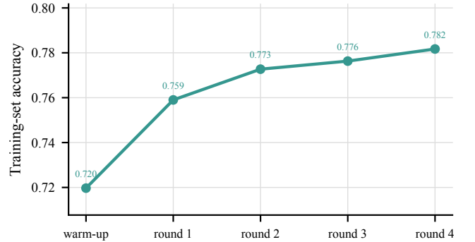
Fig. 7. Accuracy on the learning set of OGB-Arxiv across learning rounds.
