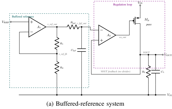
Fig. 3. The verified ldo_005_buffered_ref (Table XII), adapted from the TI TPS7A21 [48]. (a) The reference buffer A_1 and an RC low-pass filter feed the error amplifier A_2 , which drives the PMOS pass device; the output is compared directly against the filtered reference, with no output divider. (b) A_2 , a self-biased two-stage Miller OTA with a level-shifted PMOS mirror load; the high-value tie R_{EAnd} pins the otherwise floating mirror gate rail, the one-element repair of Appendix A-B. The commercial datasheet publishes only the functional block diagram; the transistor-level realizations of A_1 and A_2 are authored in this work, so the entry records an adapted re-realization, not the commercial part. In silicon the rail would be pinned by a diode-connected device or a dedicated bias branch; the resistive tie is the simulation-level equivalent, and the netlist notes record it as such.
