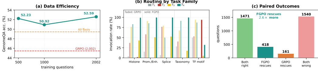
Figure 6: Additional analysis. (a) 500 training questions already beat GRPO trained on 2,002 questions and the training-free All-Tools baseline. (b) Per-tool invocation rate within each task family (Figure 4 aggregates over them). GRPO calls every tool at a similar rate whatever the question type; FGPO routes ( T_2 for TF motif, T_4 elsewhere) and never calls T_1 on any benchmark against GRPO’s 21–64%: a learned refusal. (c) FGPO rescues 2.6 \times as many questions as GRPO.
