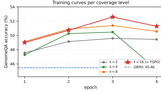
Figure 10: The coverage dial: per-epoch training curves for k \in \{2, 4, 8, 16\} actions evaluated per visit. k=16 is FGPO itself.
