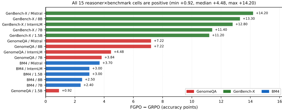
Figure 9: FGPO - GRPO for all 15 reasoner×benchmark cells, sorted. No cell is negative. Colour denotes benchmark.
