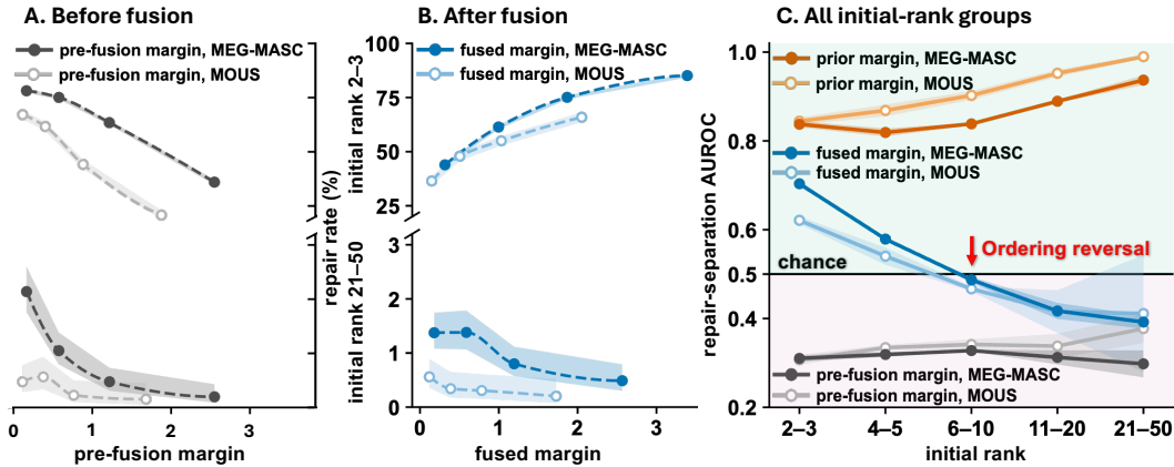
Figure 2: Confidence ordering reverses as the correct candidate starts lower in the local ranking. Initially incorrect windows on MEG-MASC (filled) and MOUS (hollow). Panels A and B use the same windows and outcomes, with one point per quartile at its mean margin; the upper and lower rows show initial ranks 2–3 and 21–50, respectively, with different vertical scales. (A) Before fusion. Repair rate decreases with margin in both groups. (B) After fusion. From the smallest to largest quartile, repair rate rises at ranks 2–3 and falls at ranks 21–50. (C) All initial-rank groups. Repair-separation AUROC of the fused, pre-fusion, and prior margins; above 0.5 favours repairs, below 0.5 residual errors. Bands are Wilson 95% intervals in A, B, and \pm 1 SD across three local decoders in C; dashed curves interpolate quartile points. MOUS ranks 21–50 average 13 repairs per decoder; Appendix E reports full rates and participant-level intervals.
