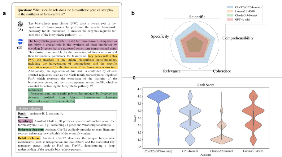
Fig. 3: Comparison results of responses from different models and ChatT2. (a) The figure shows the comparison of the response texts between the original LLM and ChatT2, which uses the same LLM as its brain, for the same question; (b) Radar chart comparing the performance of responses from ChatT2 and different models across five evaluation metrics. Violin plot illustrating the rank score distributions of responses from ChatT2 and different models.
