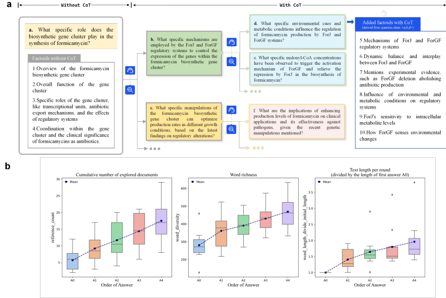
Fig. 4: The overall result of ChatT2 with CoT and without CoT between the Mentor and Executor. (a) The panel shows the questions formulated by the Mentor over multiple interaction rounds with the Executor; (b) After applying CoT techniques, the evaluation results for the answers are presented in terms of the cumulative number of explored documents, word richness, and text length per round.
