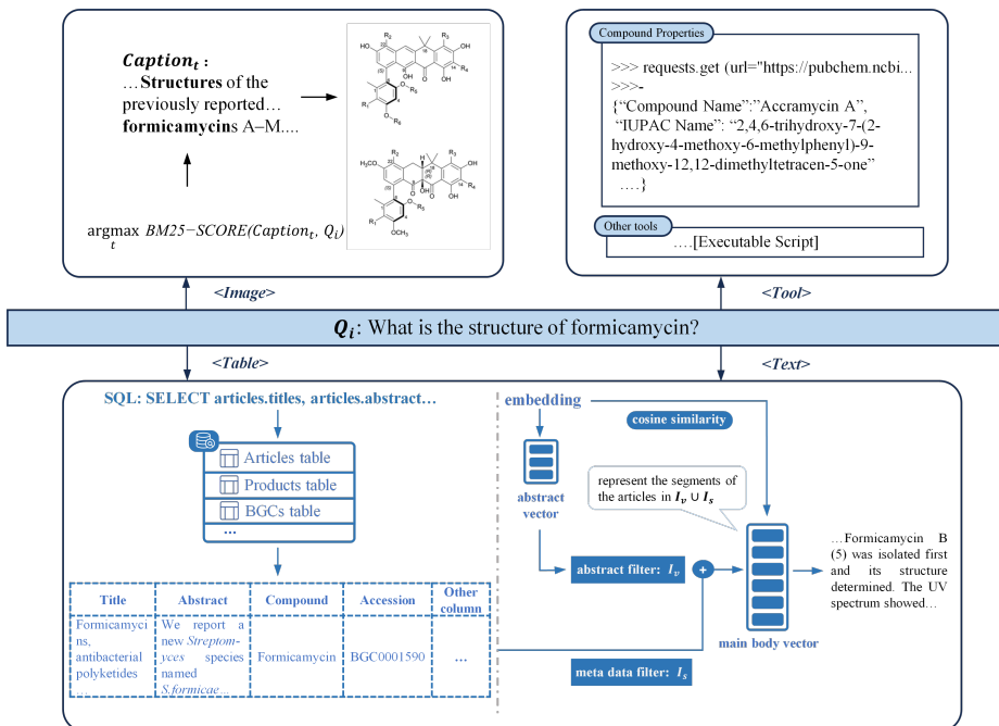
Fig. 2: Multiple retrieval source of executor. When the Executor receives a query, it transforms the query into four different types of searches across a relational database, vector database, image database, and tool repository to retrieve relevant information. Relational and Vector Databases: The query is transformed into SQL statements and text embeddings: SQL statements are executed to retrieve table information related to the query, presented within <Table> tags. During this process, relevant literature sources are gathered, forming a collection of papers denoted as I_s . Text embeddings are used to perform hierarchical semantic similarity matching based on cosine similarity. First, a semantically similar set of papers is identified, denoted as I_v . The embeddings of the query are then used to match the semantic similarity of document chunks from I_v \cup I_s , extracting text relevant to the query from the body of the papers. This information is presented within <Text> tags. Image Database: The query is matched against image titles using BM25 scores. High-scoring images are identified, and their URLs are saved as image information, presented within <Figure> tags. Tool Repository: The Executor parses key information from the query as input for prepackaged executable scripts. The execution results of these scripts are treated as tool repository information, encapsulated within <Tool> tags.
