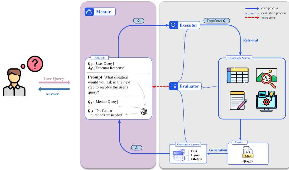
Fig. 1: The workflow of ChatT2 framework. Core process: The Mentor and Executor engage in t rounds of interaction. In each round, the Mentor submits a query to the Executor, who processes it and retrieves relevant contextual information from various knowledge bases. This information may include text, images, citations, and other supporting materials to address the current query. Based on the user’s original intent and the results returned by the Executor in previous rounds, the Mentor formulates the next query. After completing t rounds, the Mentor summarizes all the questions and answers from the interaction into a final response, which is then returned to the user. Evaluation process: The Evaluator interacts with the Executor before, during, and after the retrieval and answer generation process to enhance response quality. Raise error: If the Evaluator identifies anomalies during the Executor’s retrieval process, it reports them to the Mentor.
