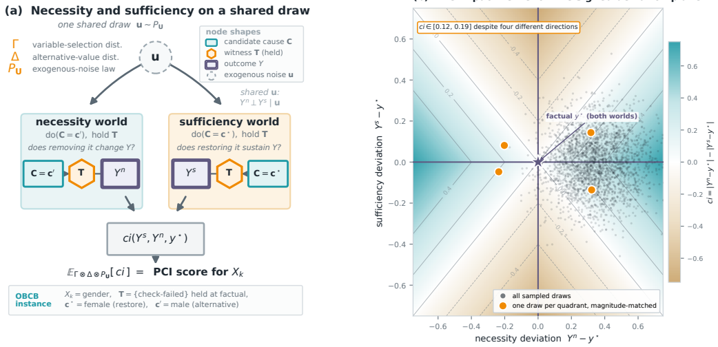
Figure 4: The PCI mechanism. (a) For a variable of interest X_k , a single exogenous draw \mathbf{u} \sim P_U together with a candidate cause set \mathbf{C} \ni X_k and witness set \mathbf{T} from \Gamma and an alternative value \mathbf{c}' from \Delta defines two counterfactual worlds on the same noise and the same (\mathbf{C}, \mathbf{T}) : a necessity world ( \text{do}(\mathbf{C} = \mathbf{c}') , witnesses held) giving Y^n , and a sufficiency world ( \text{do}(\mathbf{C} = s^*) , witnesses held) giving Y^s . Conditional on \mathbf{u} and (\mathbf{C}, \mathbf{T}) the two worlds are independent (Definition 18); the impact kernel ci scores the pair, and its expectation over \Gamma \otimes \Delta \otimes P_U (Definition 19) is PCI’s realised score. The strip grounds the schematic in the OBCB running example. (b) The impact kernel on the signed plane (Y^n - y^*, Y^s - y^*) , shown for the Absolute Difference score ci = |Y^n - y^*| - |Y^s - y^*| , one admissible choice of kernel (the PNS binary score and necessity-only variants are others), before either deviation is folded by |\cdot| . Because ci depends only on the two absolute deviations, the field is symmetric under an independent sign flip of either axis: four qualitatively different outcomes, necessity and sufficiency each landing above or below the factual value, collapse onto the same score whenever the magnitudes match. The faint cloud is a sample of (Y^n, Y^s) draws; the four gold points are actual draws, one per quadrant, with closely matched |Y^n - y^*|, |Y^s - y^*| , so their nearly equal ci values arise from the sampled data itself.
