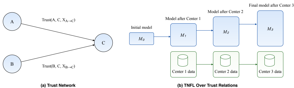
Fig. 1: Trust-constrained model propagation in TNFL. (a) Directed pairwise trust relations define which model transmissions are permitted between centers, forming the trust network over which collaboration can proceed. (b) TNFL realizes progressive cross-center learning along an admissible trust sequence. The aging-clock model is updated at each visited center, with its model capability progressively enhanced as information from more centers is incorporated.
