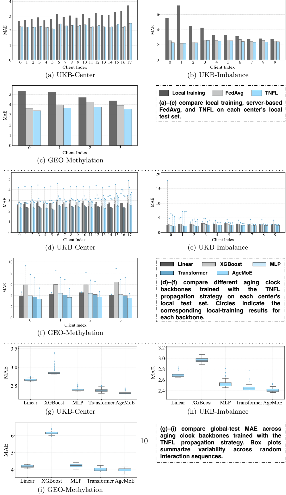
Fig. 4: Predictive performance of TNFL and its compatibility with different aging-clock backbones across multi-center datasets. Panels (a)–(c) compare TNFL with local training and server-based FedAvg, whereas panels (d)–(i) evaluate different aging-clock backbones under the TNFL propagation strategy. AgeMoE denotes the main implementation with generative replay.
