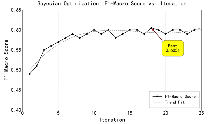
Fig. 1: Visualization of Hyperparameter Optimization Process
