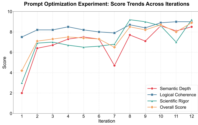
Fig. 3: prompt optimization scores
