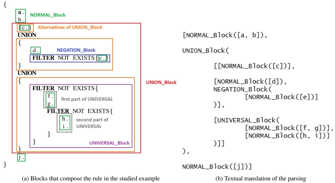
Fig. 5: Parsing of the blocks that compose the query used as example
