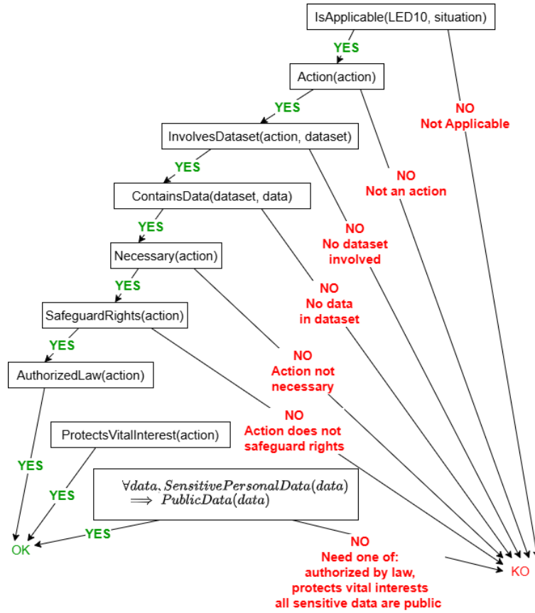
Fig. 4: Tree to determine the unfulfilled condition of the rule that checks for compliance with article 10 of the LED
