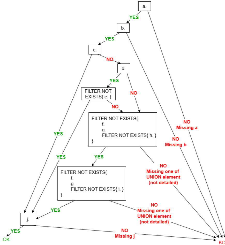
Fig. 3: Tree to determine the unfulfilled condition of the arbitrary rule from listing 2
