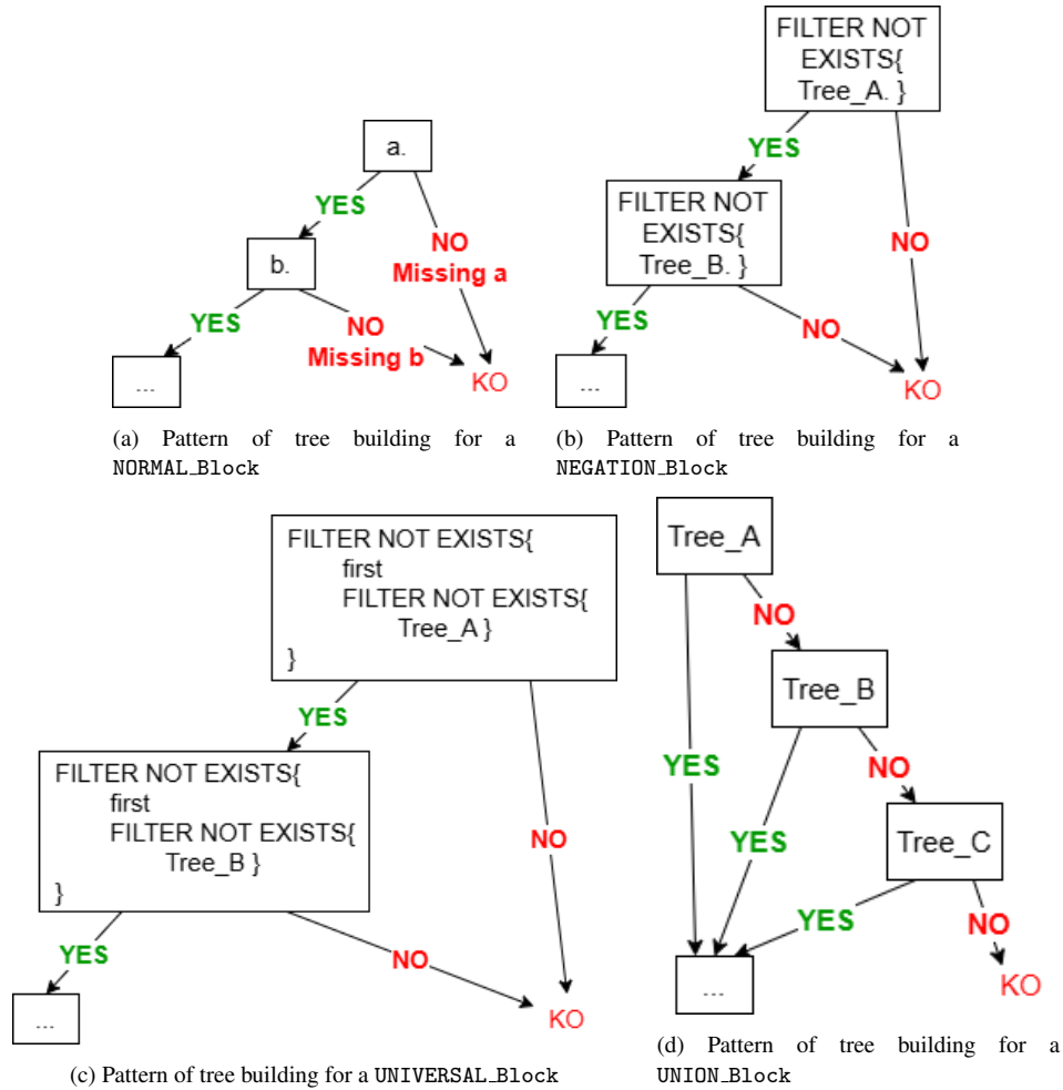
Fig. 6: Patterns of tree building depending on the type of block parsed
