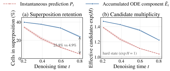
Figure 3: Candidate retention during FLM denoising. We compare the instantaneous clean prediction \mathbf{P}_t with the accumulated component \bar{\mathbf{E}}_t . (a) shows the fraction of ambiguous cells whose second-largest digit probability is at least 0.05. (b) shows the effective number of candidates, \exp(H) . The accumulated component retains more non-top-1 information than the instantaneous prediction.
