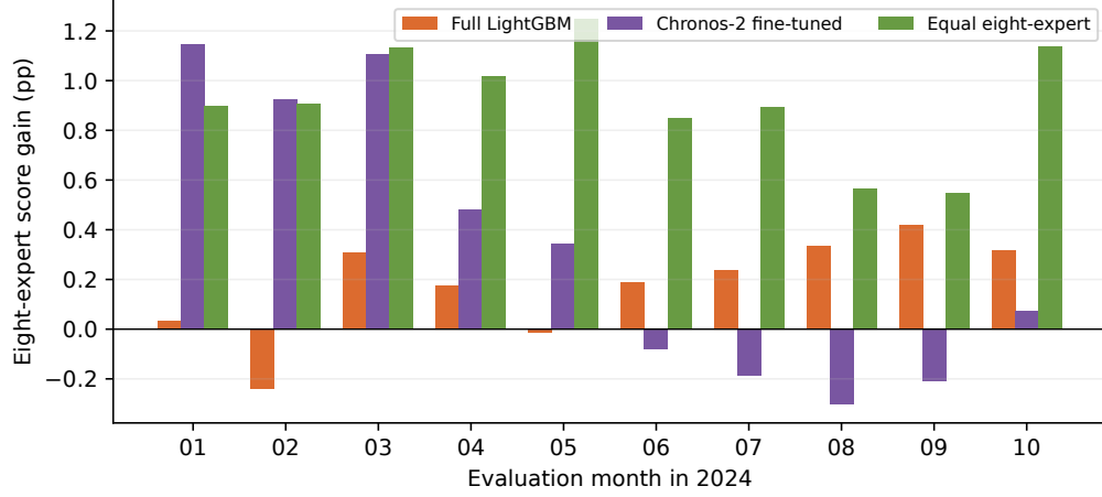
Figure 4: Monthly score gains under common calibration. Negative months are retained. The aggregate comparison does not imply dominance in each season.
