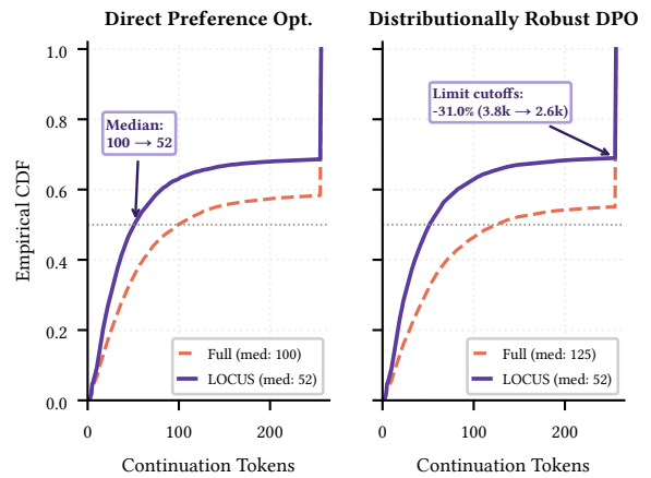
Figure 4: Continuation length CDF.
