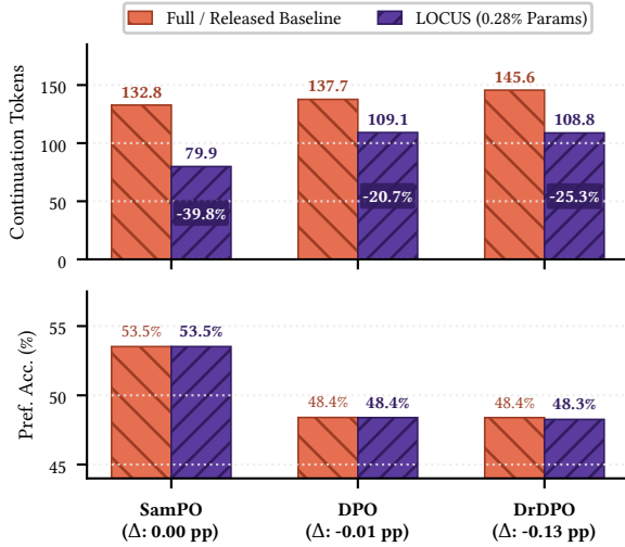
Figure 1: Token and accuracy summary on Pythia-2.8B.
