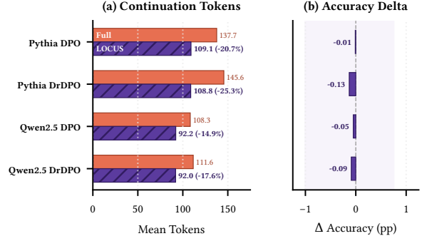
Figure 8: Cross-backbone token and accuracy results.
