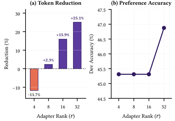
Figure 5: Sensitivity to adapter rank.
