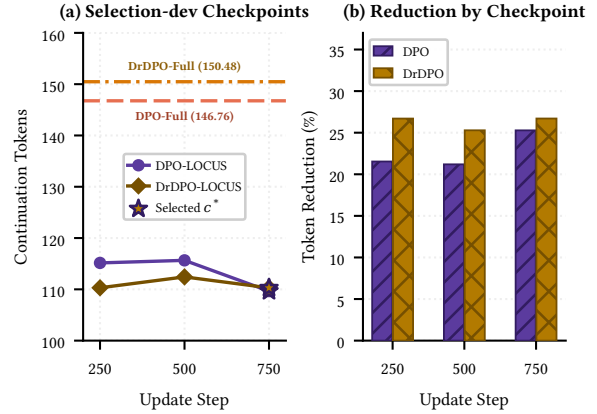
Figure 3: Constrained checkpoint selection.
