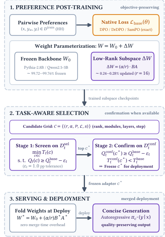
Figure 2: LOCUS procedure from native-objective training to selected low-rank deployment.
