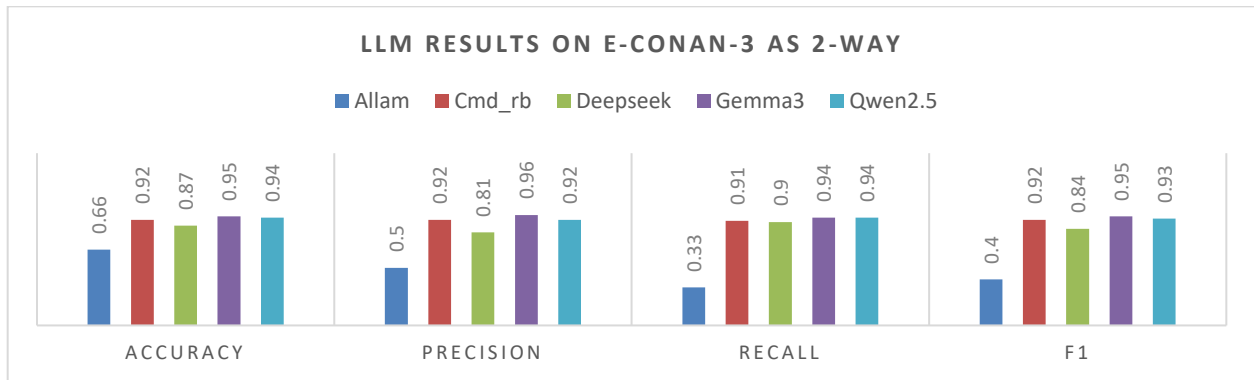
Figure11: LLM Zero-Shot Classification on E-CONAN-3 as 2-way
