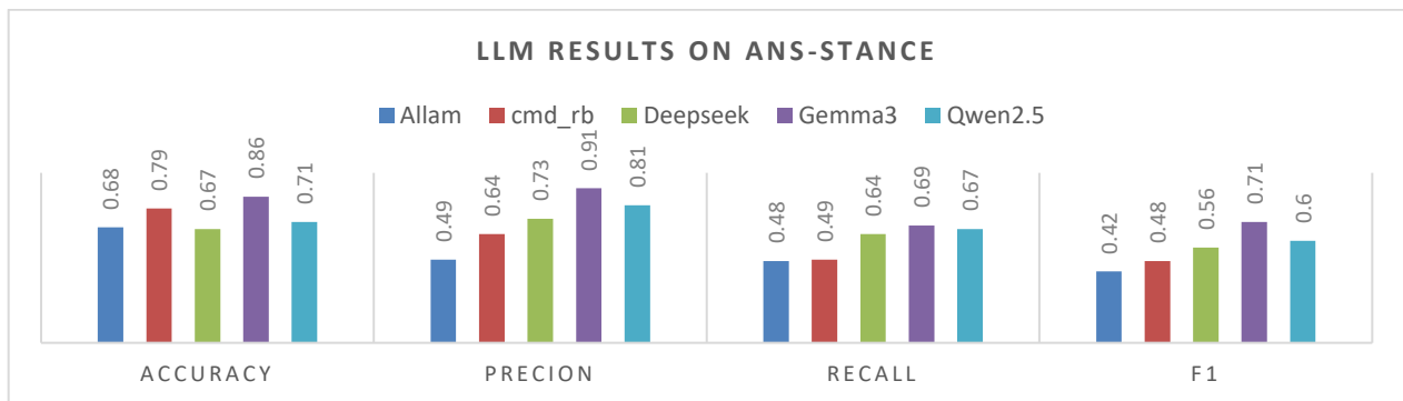
Figure12: LLM Zero-Shot Classification on Ans-Stance Dataset
