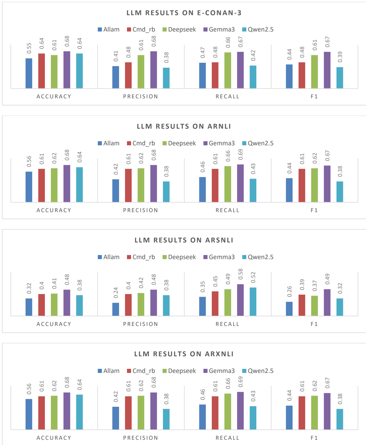
Figure13: LLM Zero-Shot Classification on E-CONAN-3 and SoTA Benchmarks
