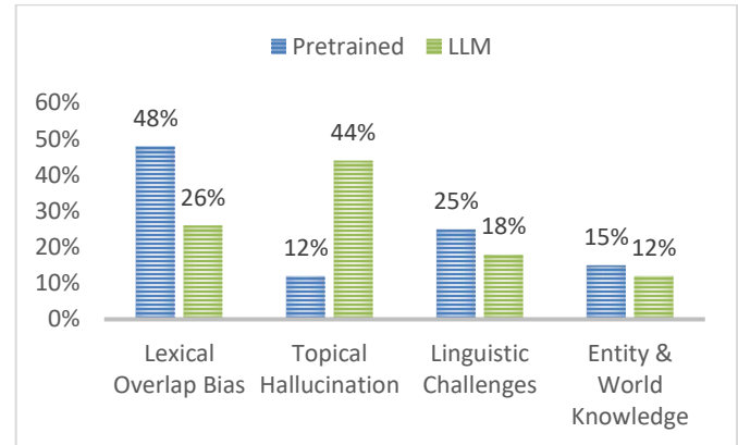
Figure14: Quantitative Error Analysis
