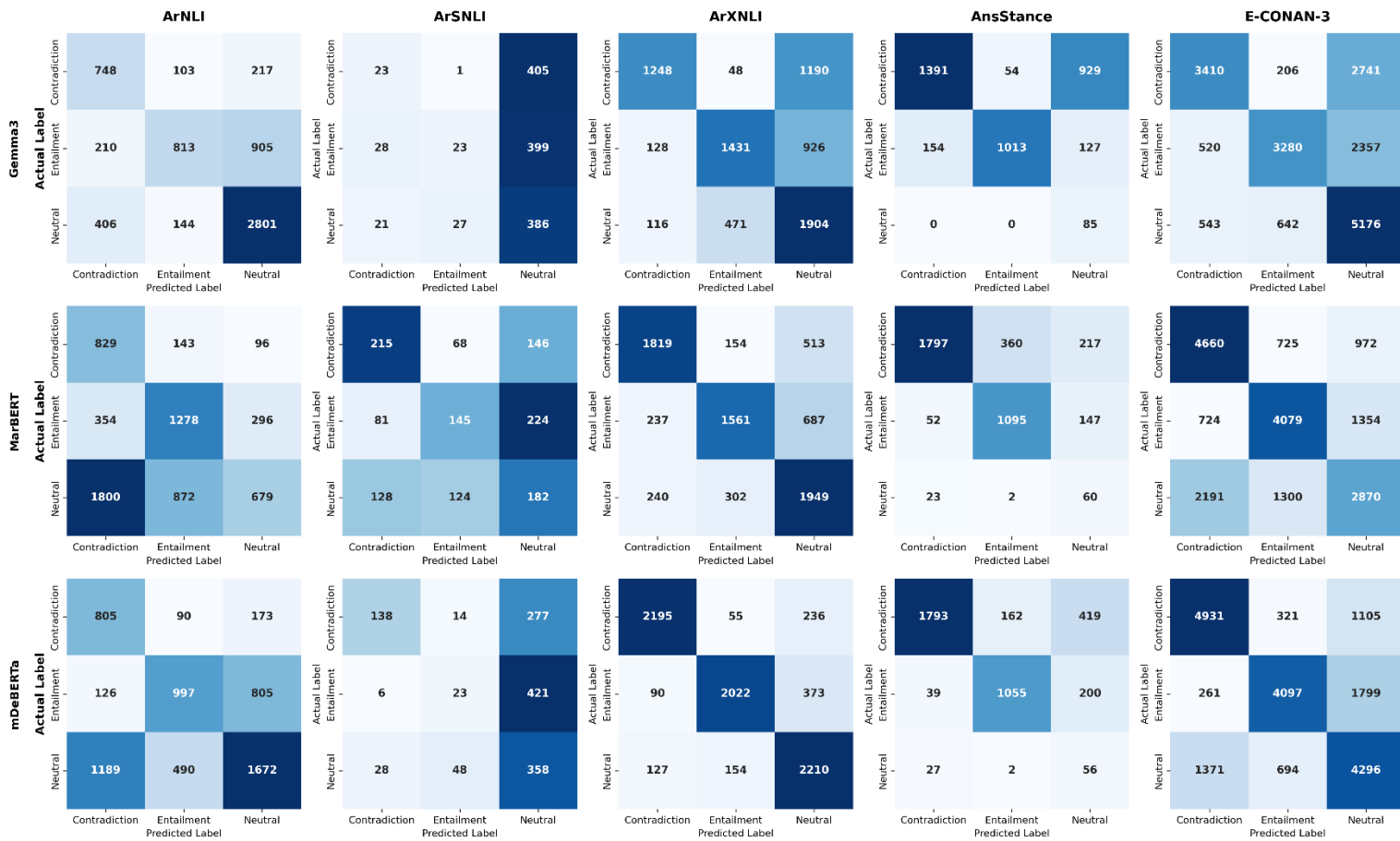
Figure15: Confusion Matrix of E-CONAN and SoTA Benchmarks
