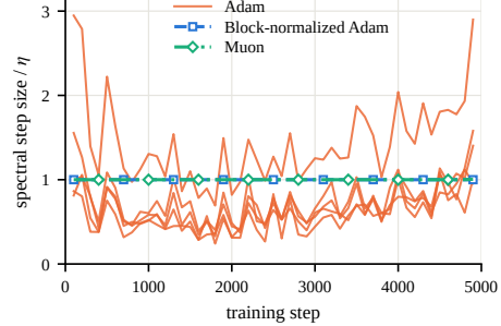
Figure 2: Spectral step divided by \eta on rMD17. Each Adam curve is one irrep block; block-normalized Adam and Muon remain at spectral step \eta .
