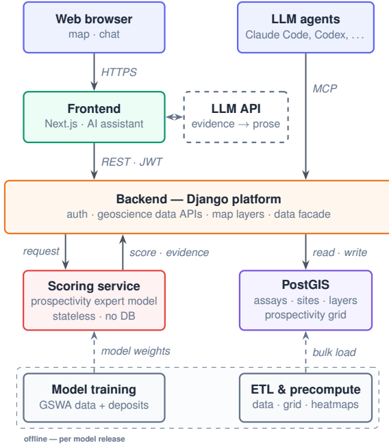
Figure 2: Architecture design for MINETRACE. Django is a Python web framework; PostGIS is a database for geospatial data; ETL means extract–transform–load for data preparation; MCP (Model Context Protocol) lets external agents call software tools.
