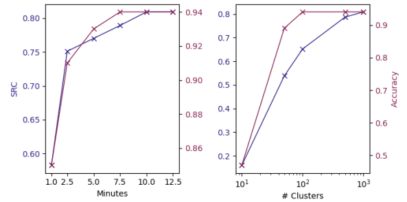
Figure 4: Effect of cluster size and number of minutes input on alignment distance SRC and classification accuracy.
