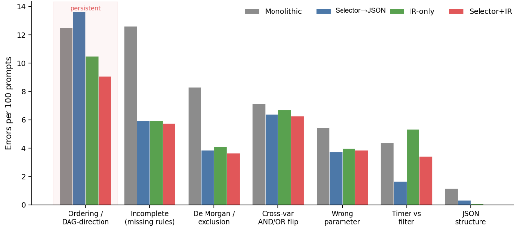
Figure 2: Error prevalence (per 100 prompts) by category and configuration, from automated coding of the judge’s rationales. Completeness/syntax categories (Incomplete, De Morgan, JSON) collapse under the pipelines; logic/topology categories (cross-variable AND/OR, Ordering) persist. Ordering—wrong DAG edge direction—is the largest and most stubborn residual. Source: Microsoft.
