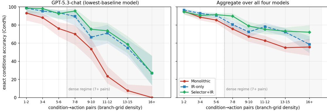
Figure 1: Exact-conditions accuracy (corrected scorer) vs. branch-grid density (condition→action pairs). Left: GPT-5.3-chat; right: aggregate over all four models. Shaded bands are Wilson 95% CIs. Monolithic generation collapses on dense rules while the compiler configurations degrade gracefully—the visual signature of the emission-density bottleneck. Source: Microsoft.
