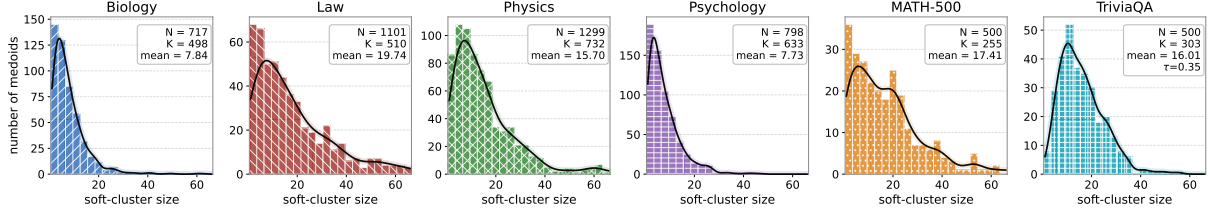
Figure 1: Soft-cluster size distribution (members per medoid under POOL’s attention rule) for all benchmarks. Heavier right tails (Law, Physics, MATH-500) reflect denser topical redundancy and translate directly into higher POOL compression (Table 5). Psychology has the lightest tail and correspondingly the smallest savings.
