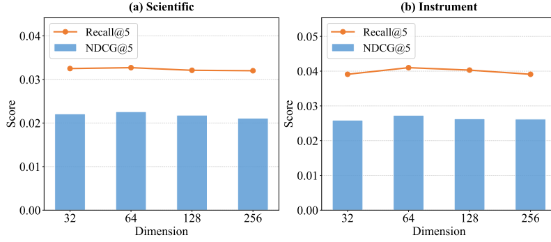
Fig. 7. Hyper-parameter study with different dimensionalities for collaborative embedding.
