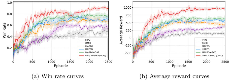
Fig. 3: Training curves of DRG-MAPPO and other baselines in the 2v2 scenario.
