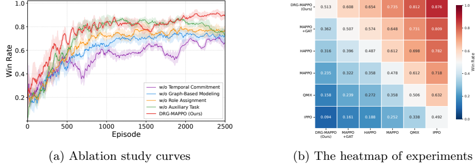
Fig. 4: Comprehensive evaluation in the 2v2 scenario. (a) The training win rates of ablation experiments. (b) The heatmap of confrontation experiments.
