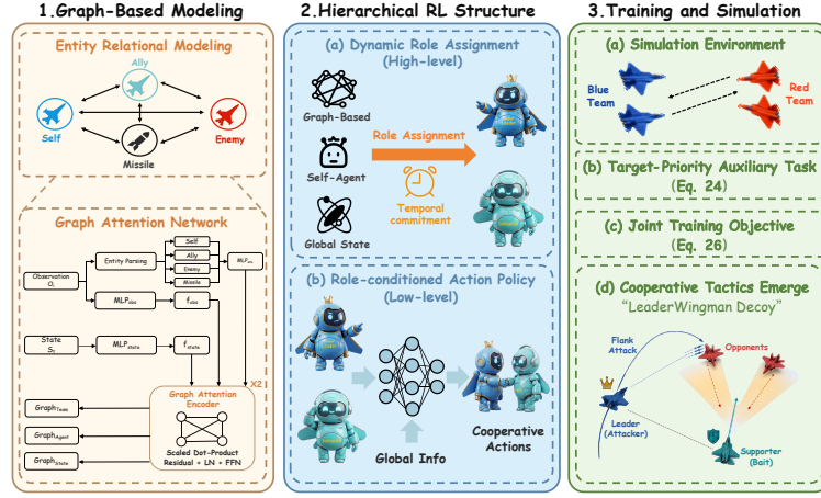
Fig. 2: Overview of the DRG-MAPPO framework. (1) graph-based state modeling for entity relationship extraction, (2) a hierarchical RL structure for tactical decision-making, and (3) centralized training and decentralized simulation.
