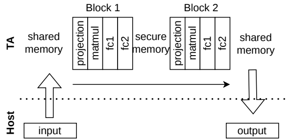
Figure 5: Inference of two consecutive blocks in the TA. The input gets sent to the TA as a pointer to shared memory. Working memory and block results are kept in secure memory, except for the outputs of the last block, which gets placed into shared memory. The shared memory pointer gets passed to the host as the output, which can read the result.
